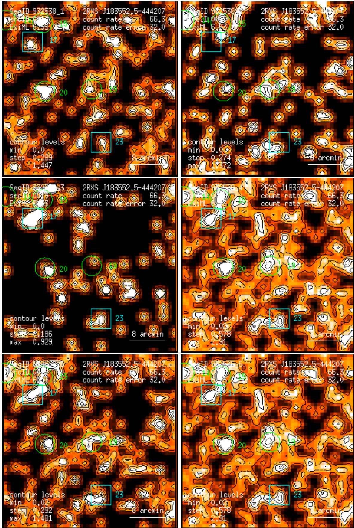
Figure 19: RASS 932538: detection 0019: band rate images, Gaussian filter: (1) PSPC channels 11 – 41, (2) 52 – 90, (3) 91 – 201, (4) 11 – 235, (5) 52 – 201, (6) 11 – 201. Broad band rates in counts/ks. Band rate contour levels in counts/ks/arcmin 2 .
