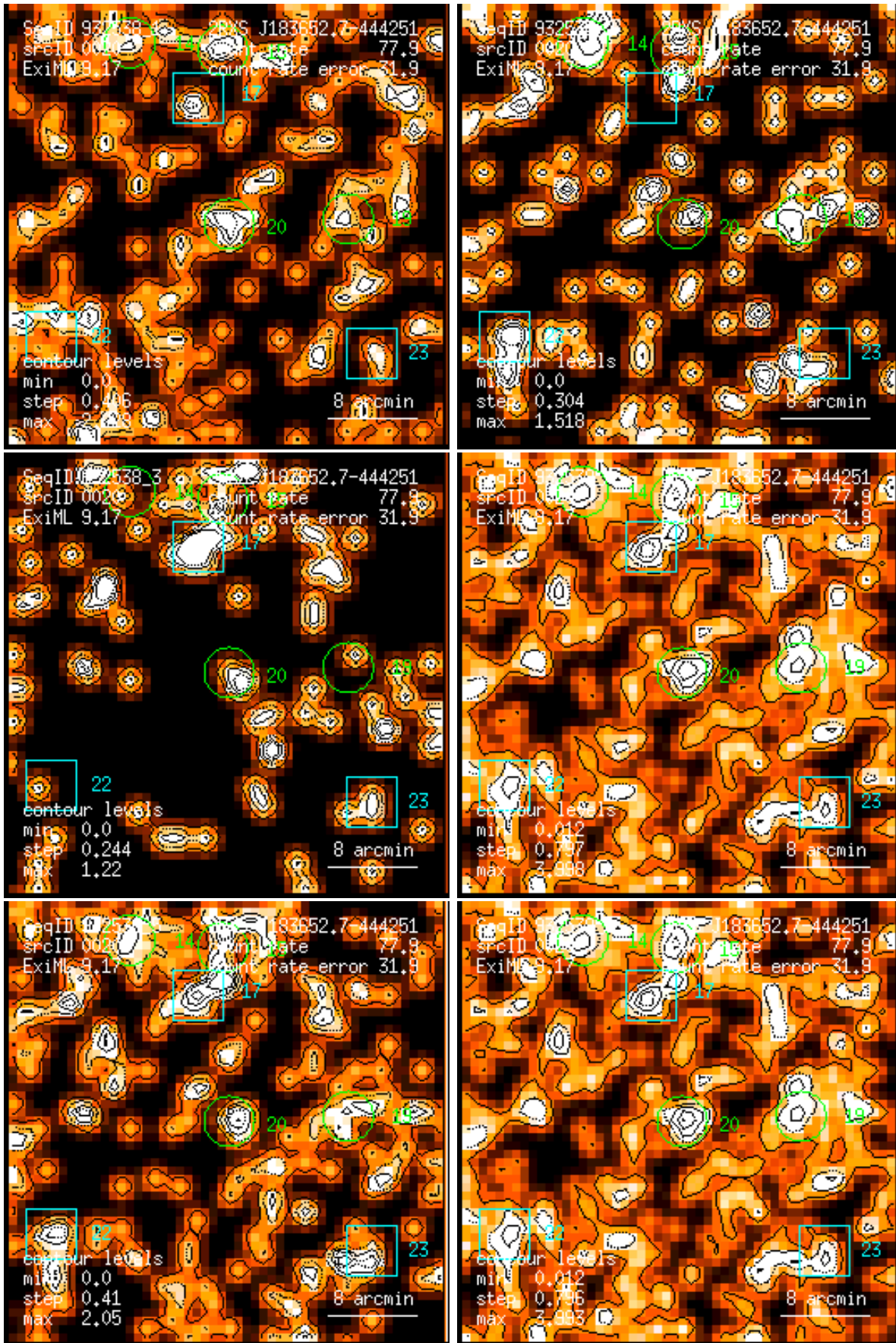
Figure 20: RASS 932538: detection 0020: band rate images, Gaussian filter: (1) PSPC channels 11 – 41, (2) 52 – 90, (3) 91 – 201, (4) 11 – 235, (5) 52 – 201, (6) 11 – 201. Broad band rates in counts/ks. Band rate contour levels in counts/ks/arcmin 2 .
