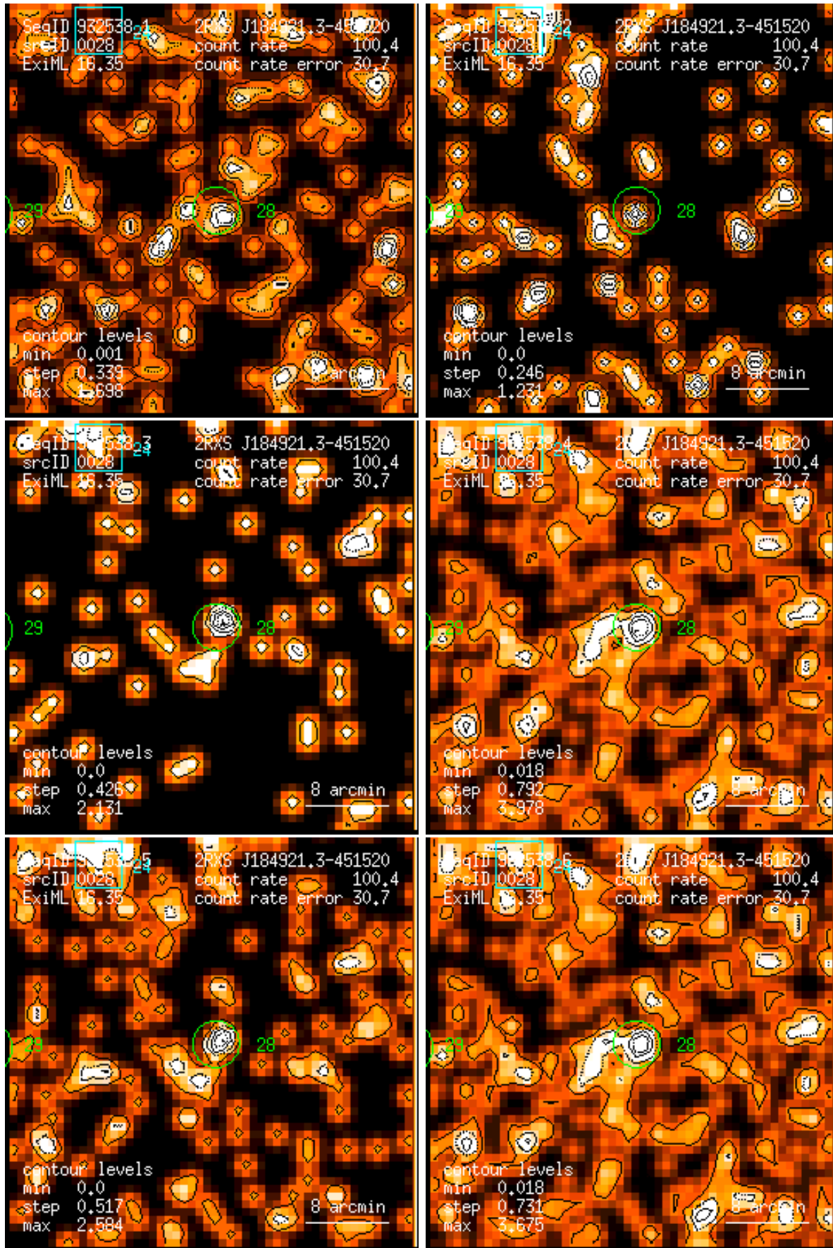
Figure 28: RASS 932538: detection 0028: band rate images, Gaussian filter: (1) PSPC channels 11 – 41, (2) 52 – 90, (3) 91 – 201, (4) 11 – 235, (5) 52 – 201, (6) 11 – 201. Broad band rates in counts/ks. Band rate contour levels in counts/ks/arcmin 2 .
