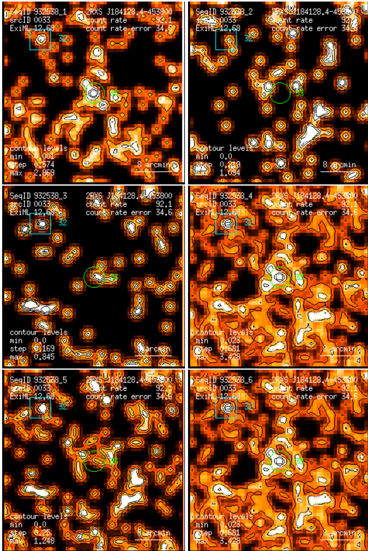
Figure 33: RASS 932538: detection 0033: band rate images, Gaussian filter: (1) PSPC channels 11 – 41, (2) 52 – 90, (3) 91 – 201, (4) 11 – 235, (5) 52 – 201, (6) 11 – 201. Broad band rates in counts/ks. Band rate contour levels in counts/ks/arcmin 2 .
