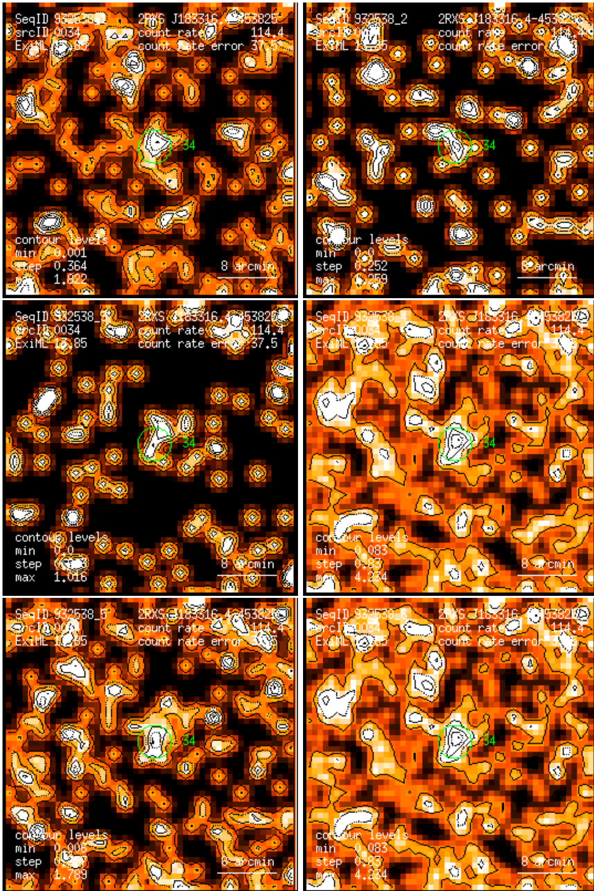
Figure 34: RASS 932538: detection 0034: band rate images, Gaussian filter: (1) PSPC channels 11 – 41, (2) 52 – 90, (3) 91 – 201, (4) 11 – 235, (5) 52 – 201, (6) 11 – 201. Broad band rates in counts/ks. Band rate contour levels in counts/ks/arcmin 2 .
