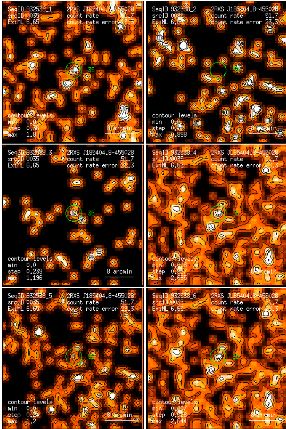
Figure 35: RASS 932538: detection 0035: band rate images, Gaussian filter: (1) PSPC channels 11 – 41, (2) 52 – 90, (3) 91 – 201, (4) 11 – 235, (5) 52 – 201, (6) 11 – 201. Broad band rates in counts/ks. Band rate contour levels in counts/ks/arcmin 2 .
