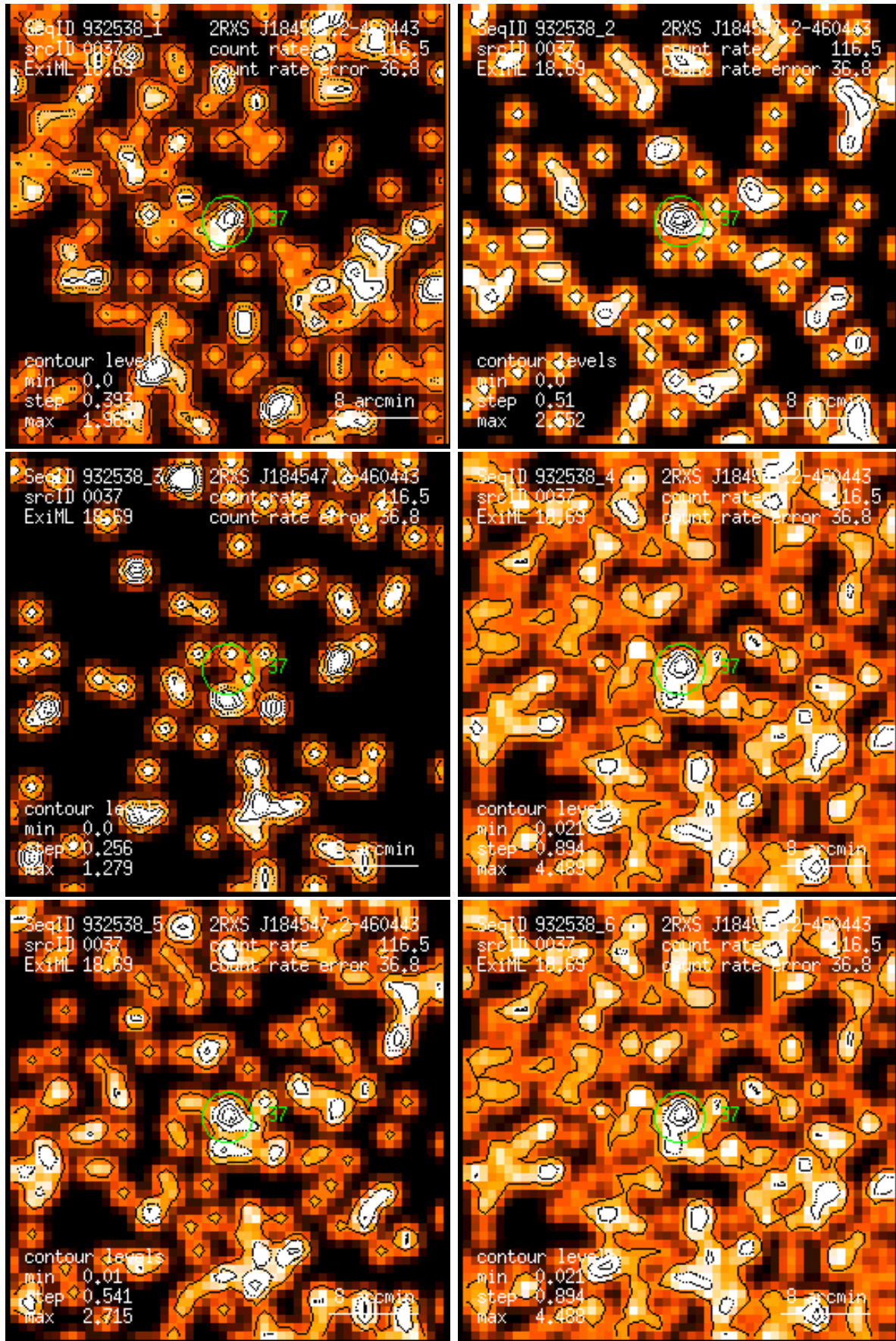
Figure 37: RASS 932538: detection 0037: band rate images, Gaussian filter: (1) PSPC channels 11 – 41, (2) 52 – 90, (3) 91 – 201, (4) 11 – 235, (5) 52 – 201, (6) 11 – 201. Broad band rates in counts/ks. Band rate contour levels in counts/ks/arcmin 2 .
