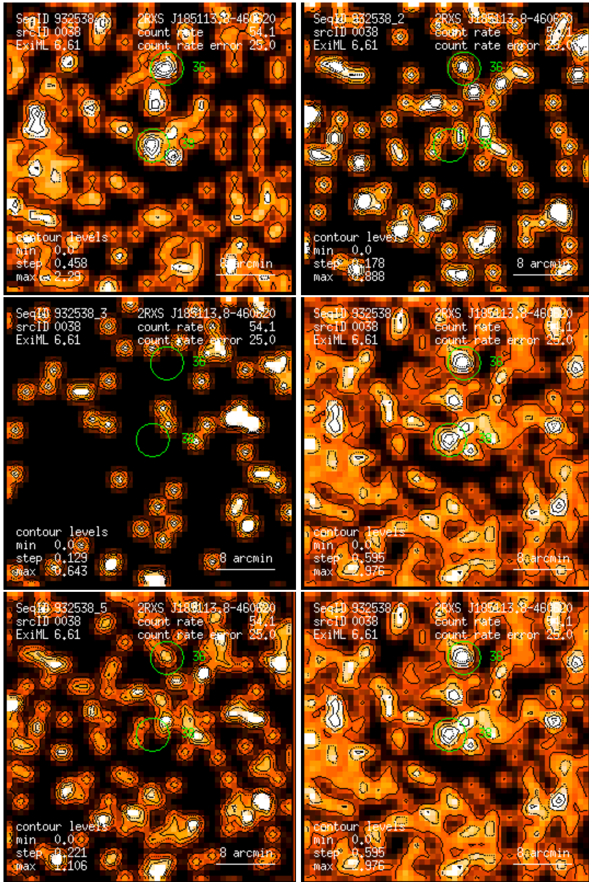
Figure 38: RASS 932538: detection 0038: band rate images, Gaussian filter: (1) PSPC channels 11 – 41, (2) 52 – 90, (3) 91 – 201, (4) 11 – 235, (5) 52 – 201, (6) 11 – 201. Broad band rates in counts/ks. Band rate contour levels in counts/ks/arcmin 2 .
