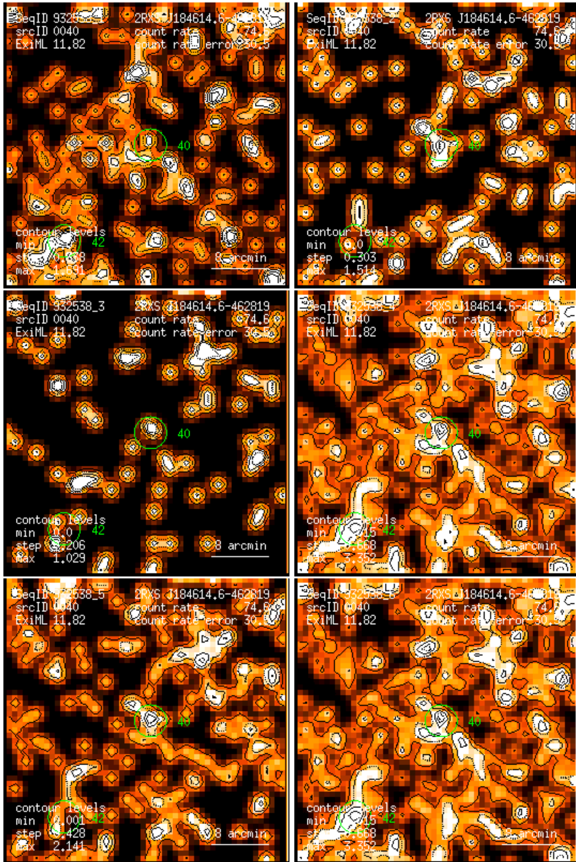
Figure 40: RASS 932538: detection 0040: band rate images, Gaussian filter: (1) PSPC channels 11 – 41, (2) 52 – 90, (3) 91 – 201, (4) 11 – 235, (5) 52 – 201, (6) 11 – 201. Broad band rates in counts/ks. Band rate contour levels in counts/ks/arcmin 2 .
