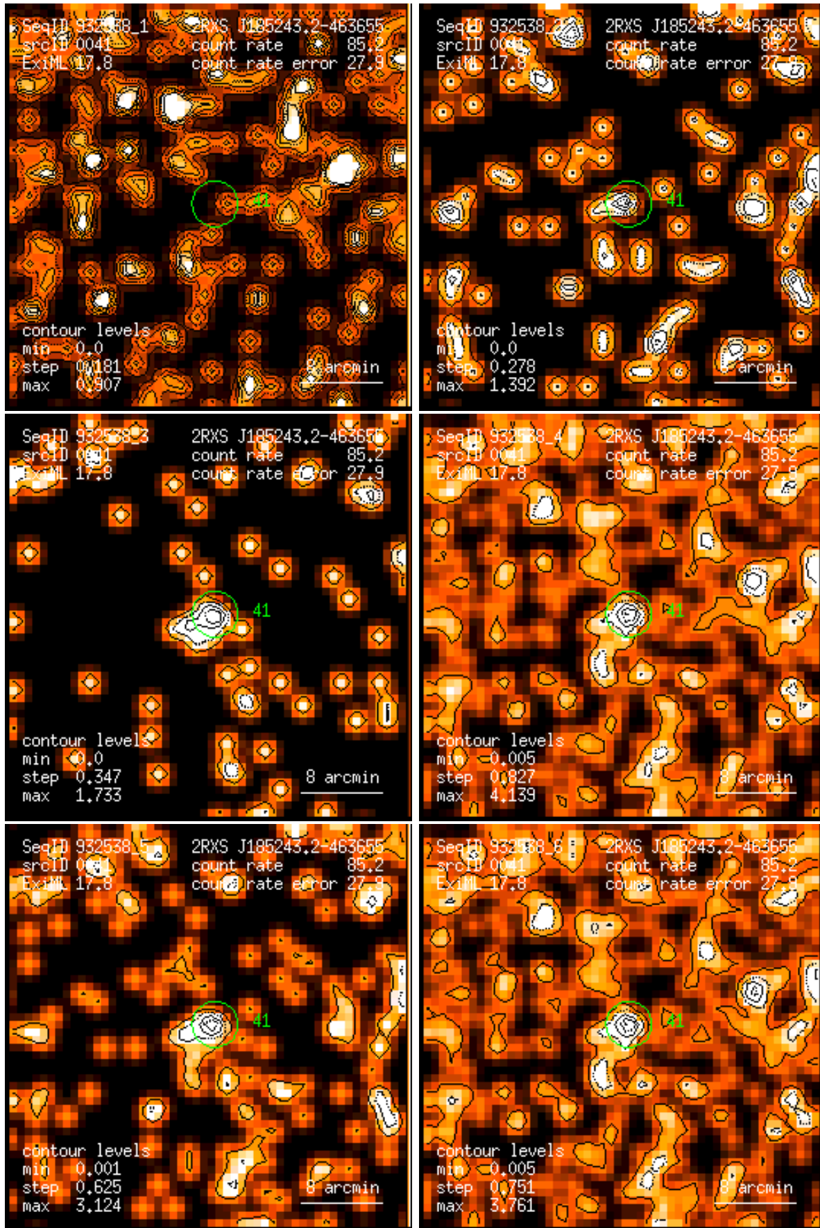
Figure 41: RASS 932538: detection 0041: band rate images, Gaussian filter: (1) PSPC channels 11 – 41, (2) 52 – 90, (3) 91 – 201, (4) 11 – 235, (5) 52 – 201, (6) 11 – 201. Broad band rates in counts/ks. Band rate contour levels in counts/ks/arcmin 2 .
