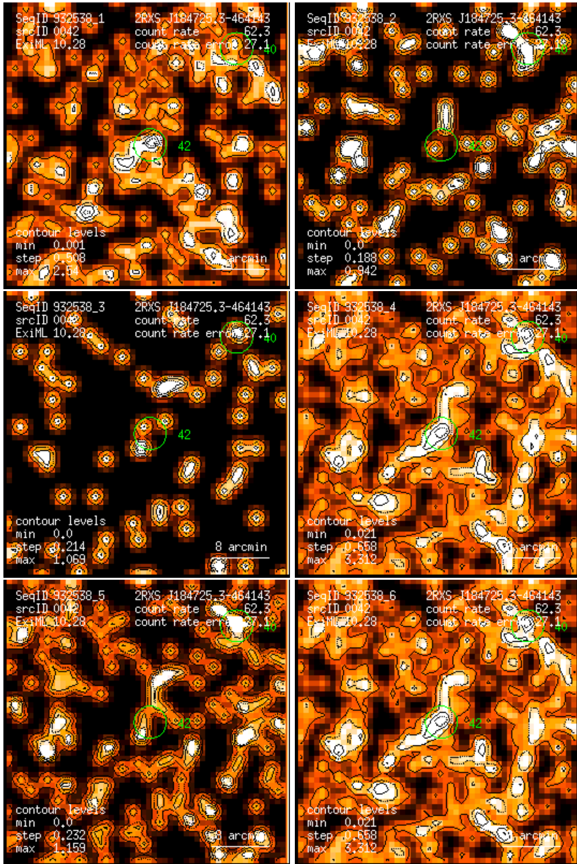
Figure 42: RASS 932538: detection 0042: band rate images, Gaussian filter: (1) PSPC channels 11 – 41, (2) 52 – 90, (3) 91 – 201, (4) 11 – 235, (5) 52 – 201, (6) 11 – 201. Broad band rates in counts/ks. Band rate contour levels in counts/ks/arcmin 2 .
