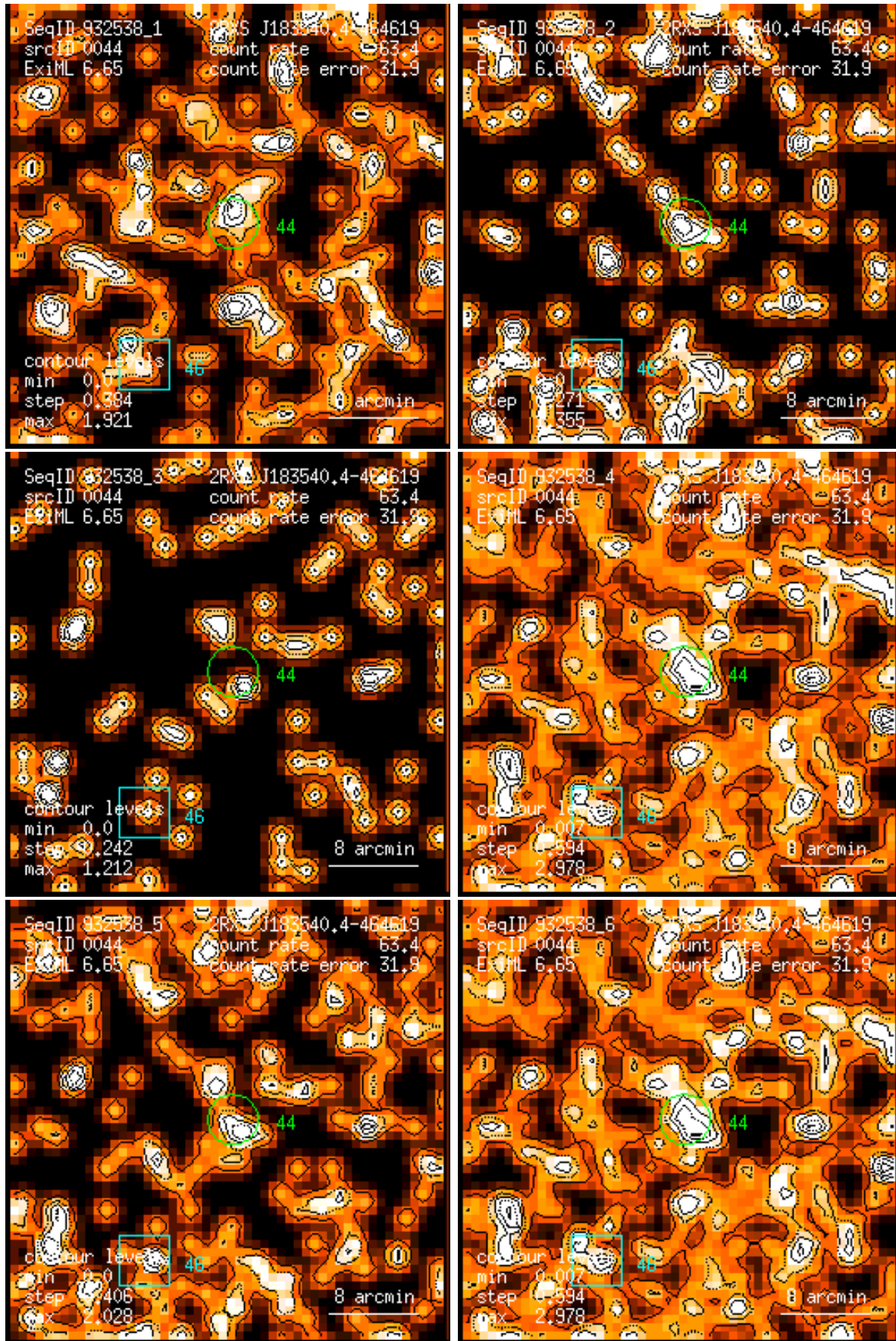
Figure 44: RASS 932538: detection 0044: band rate images, Gaussian filter: (1) PSPC channels 11 – 41, (2) 52 – 90, (3) 91 – 201, (4) 11 – 235, (5) 52 – 201, (6) 11 – 201. Broad band rates in counts/ks. Band rate contour levels in counts/ks/arcmin 2 .
