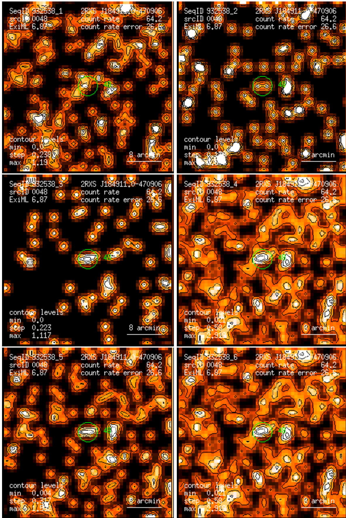
Figure 48: RASS 932538: detection 0048: band rate images, Gaussian filter: (1) PSPC channels 11 – 41, (2) 52 – 90, (3) 91 – 201, (4) 11 – 235, (5) 52 – 201, (6) 11 – 201. Broad band rates in counts/ks. Band rate contour levels in counts/ks/arcmin 2 .
