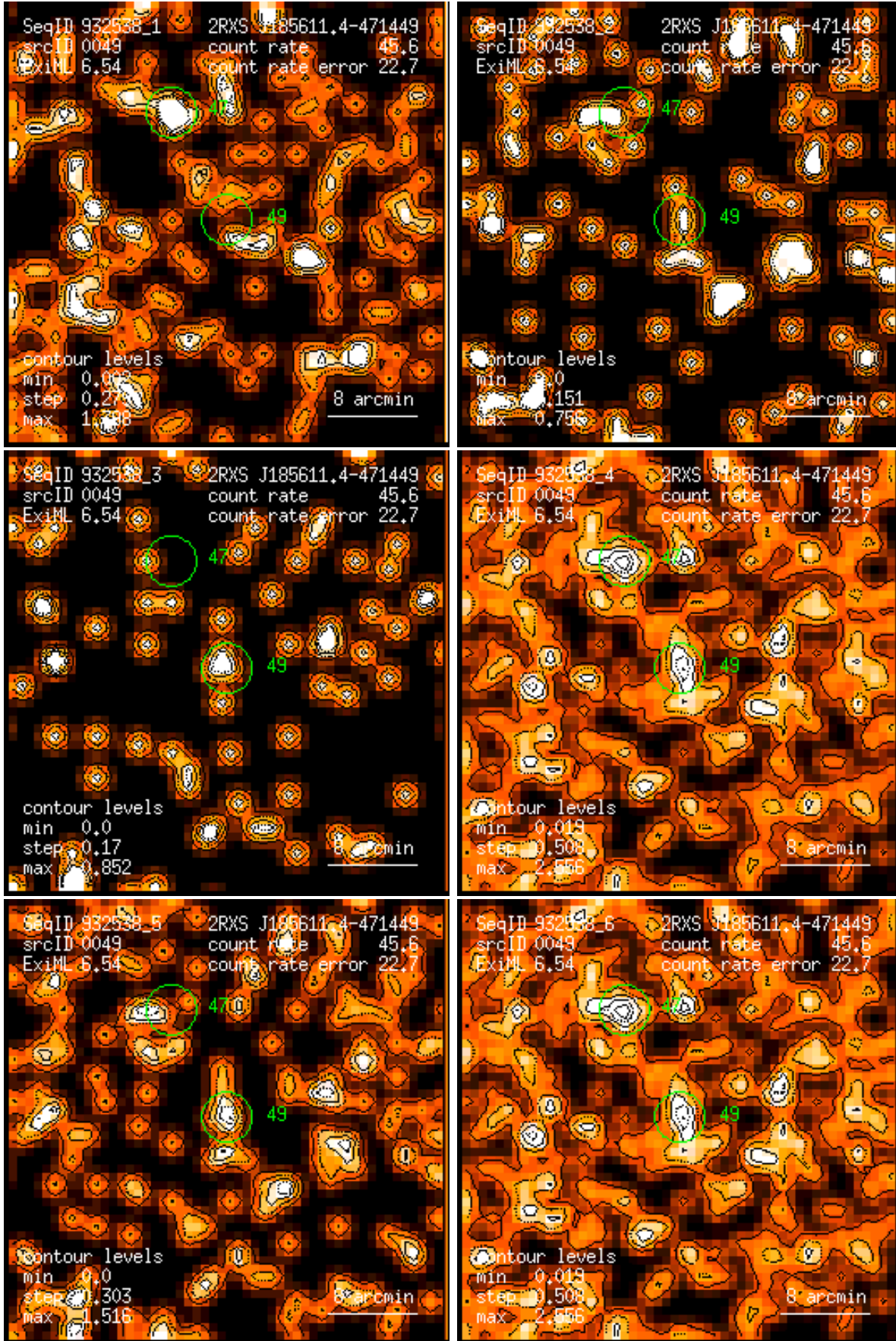
Figure 49: RASS 932538: detection 0049: band rate images, Gaussian filter: (1) PSPC channels 11 – 41, (2) 52 – 90, (3) 91 – 201, (4) 11 – 235, (5) 52 – 201, (6) 11 – 201. Broad band rates in counts/ks. Band rate contour levels in counts/ks/arcmin 2 .
