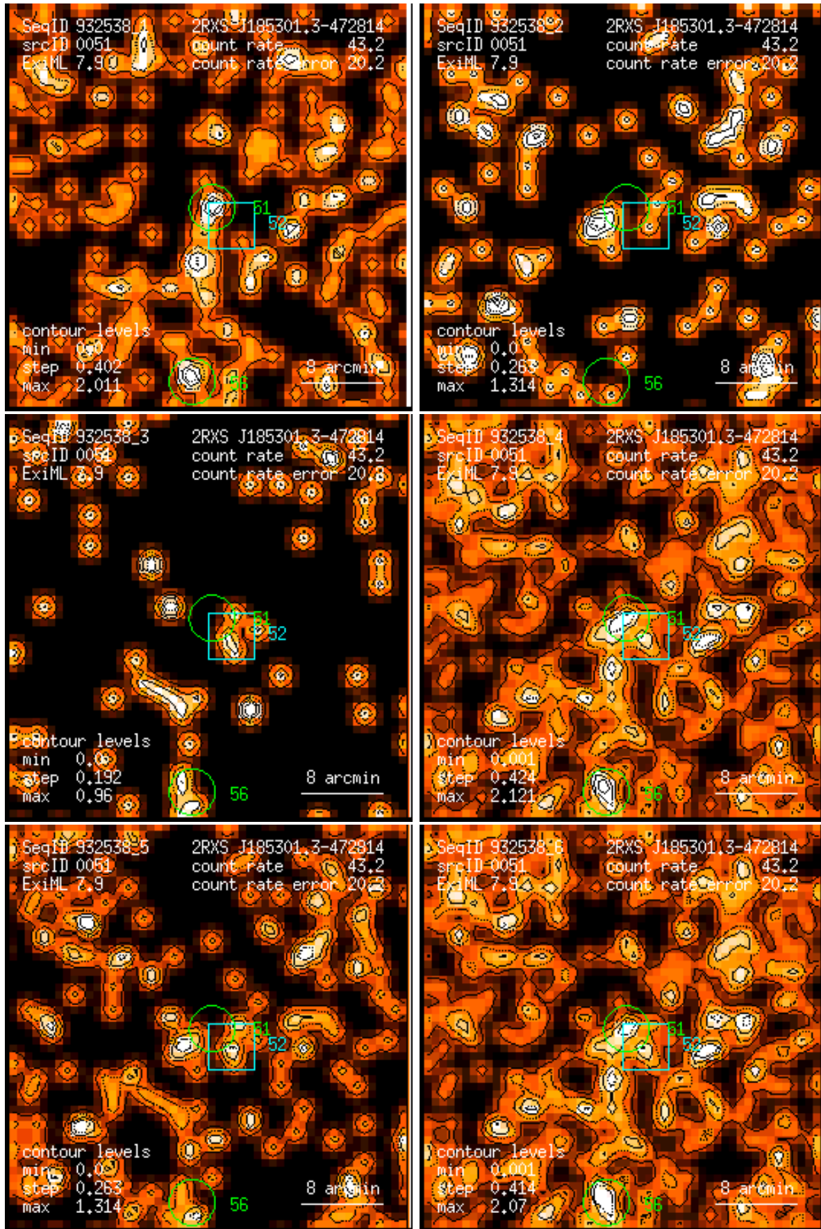
Figure 51: RASS 932538: detection 0051: band rate images, Gaussian filter: (1) PSPC channels 11 – 41, (2) 52 – 90, (3) 91 – 201, (4) 11 – 235, (5) 52 – 201, (6) 11 – 201. Broad band rates in counts/ks. Band rate contour levels in counts/ks/arcmin 2 .
