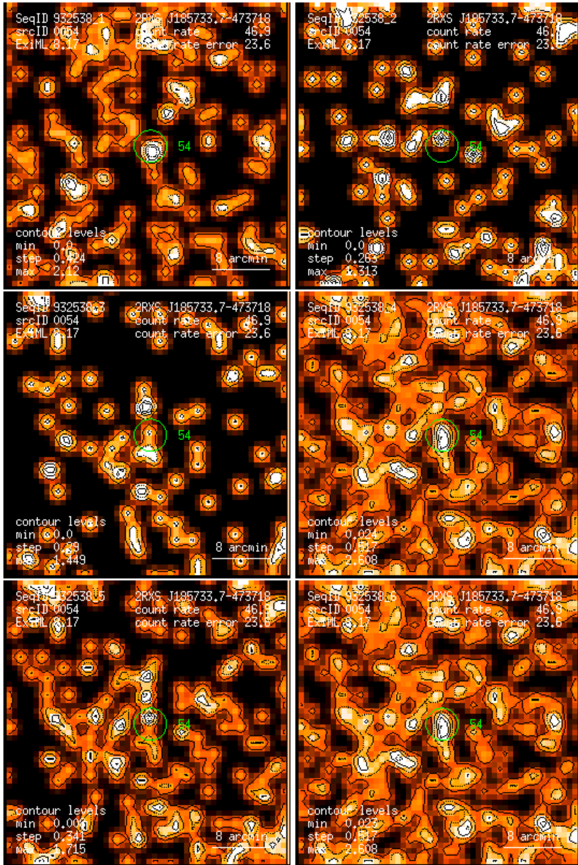
Figure 54: RASS 932538: detection 0054: band rate images, Gaussian filter: (1) PSPC channels 11 – 41, (2) 52 – 90, (3) 91 – 201, (4) 11 – 235, (5) 52 – 201, (6) 11 – 201. Broad band rates in counts/ks. Band rate contour levels in counts/ks/arcmin 2 .
