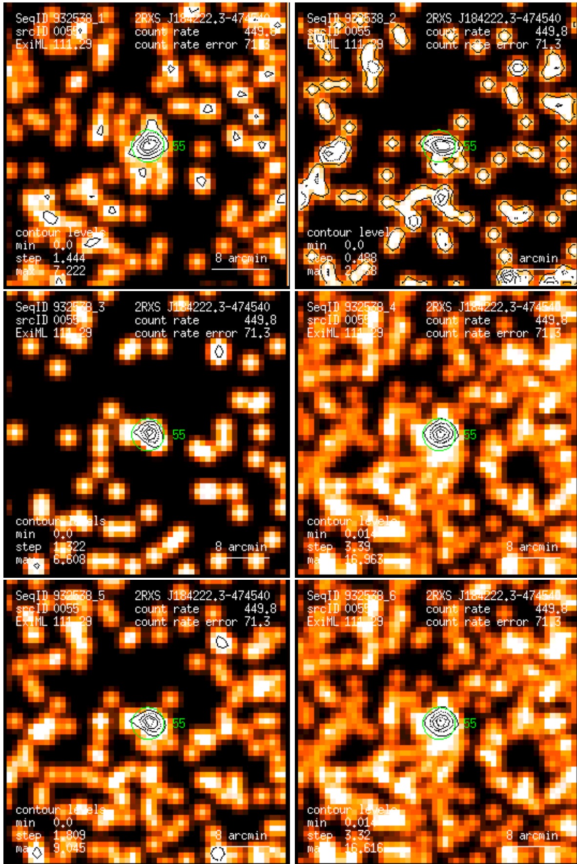
Figure 55: RASS 932538: detection 0055: band rate images, Gaussian filter: (1) PSPC channels 11 – 41, (2) 52 – 90, (3) 91 – 201, (4) 11 – 235, (5) 52 – 201, (6) 11 – 201. Broad band rates in counts/ks. Band rate contour levels in counts/ks/arcmin 2 .
