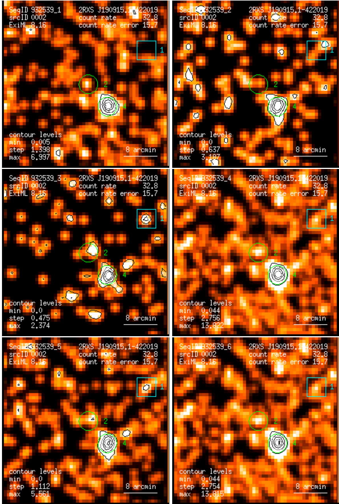
Figure 2: RASS 932539: detection 0002: band rate images, Gaussian filter: (1) PSPC channels 11 – 41, (2) 52 – 90, (3) 91 – 201, (4) 11 – 235, (5) 52 – 201, (6) 11 – 201. Broad band rates in counts/ks. Band rate contour levels in counts/ks/arcmin 2 .
