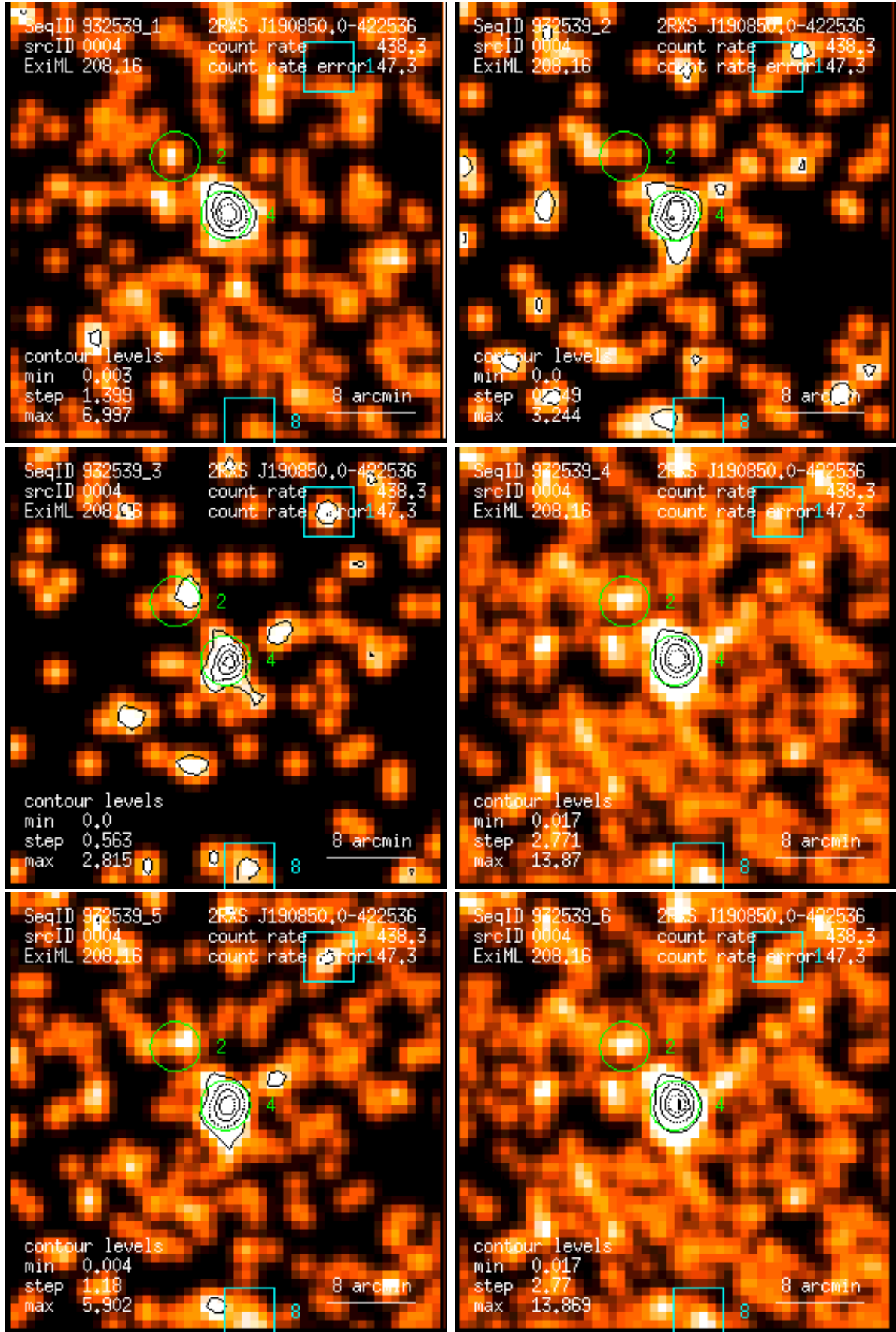
Figure 4: RASS 932539: detection 0004: band rate images, Gaussian filter: (1) PSPC channels 11 – 41, (2) 52 – 90, (3) 91 – 201, (4) 11 – 235, (5) 52 – 201, (6) 11 – 201. Broad band rates in counts/ks. Band rate contour levels in counts/ks/arcmin 2 .
