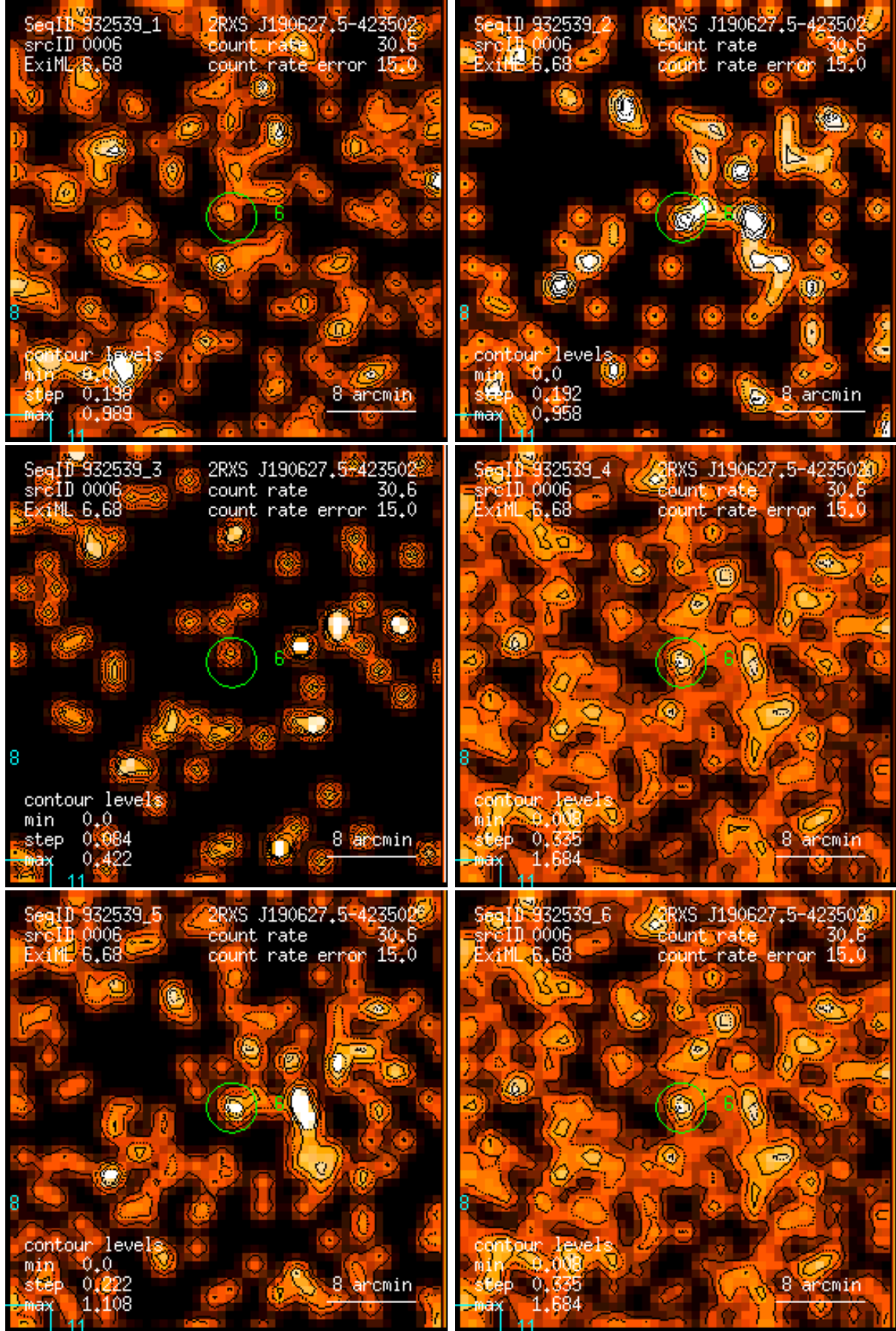
Figure 6: RASS 932539: detection 0006: band rate images, Gaussian filter: (1) PSPC channels 11 – 41, (2) 52 – 90, (3) 91 – 201, (4) 11 – 235, (5) 52 – 201, (6) 11 – 201. Broad band rates in counts/ks. Band rate contour levels in counts/ks/arcmin 2 .
