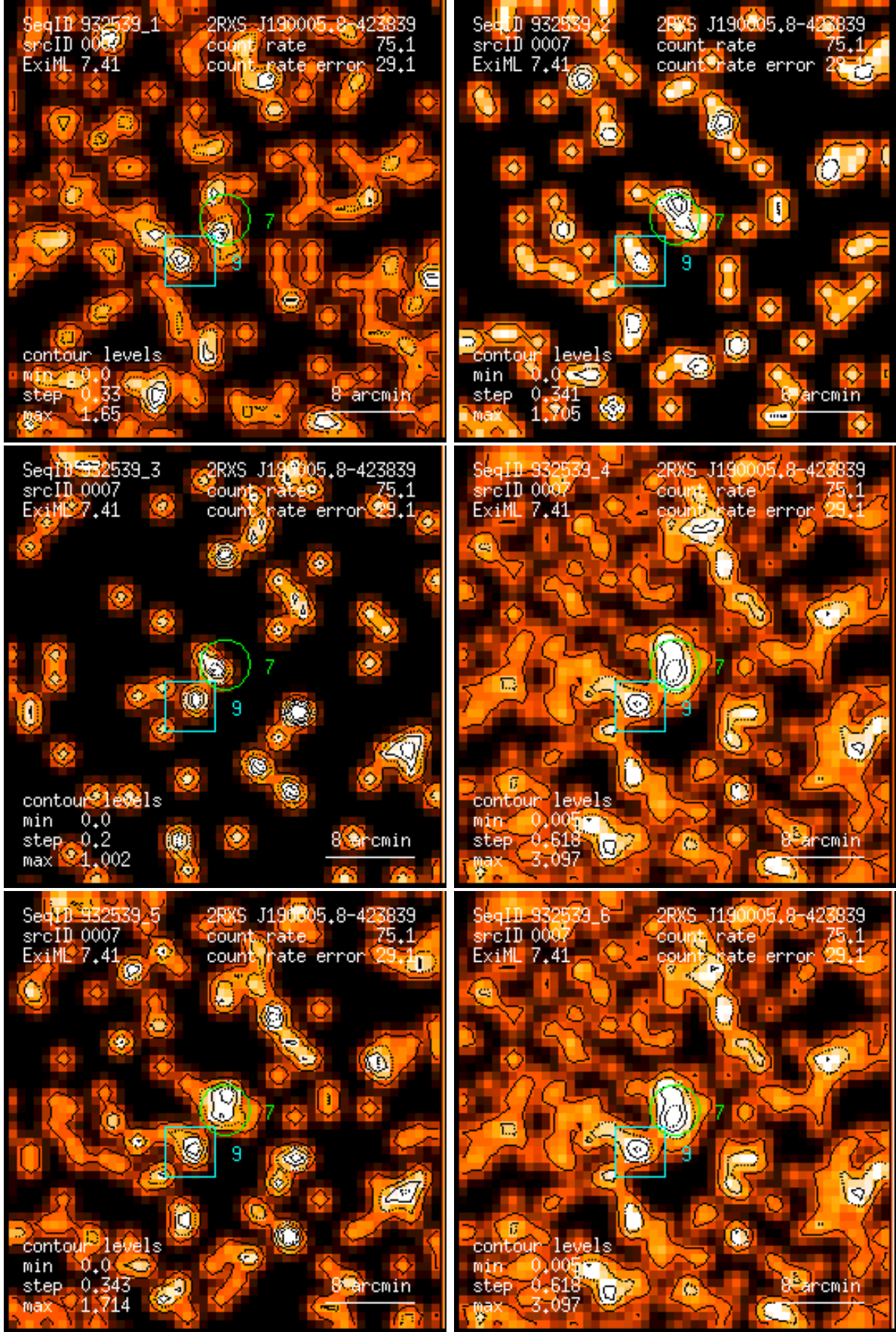
Figure 7: RASS 932539: detection 0007: band rate images, Gaussian filter: (1) PSPC channels 11 – 41, (2) 52 – 90, (3) 91 – 201, (4) 11 – 235, (5) 52 – 201, (6) 11 – 201. Broad band rates in counts/ks. Band rate contour levels in counts/ks/arcmin 2 .
