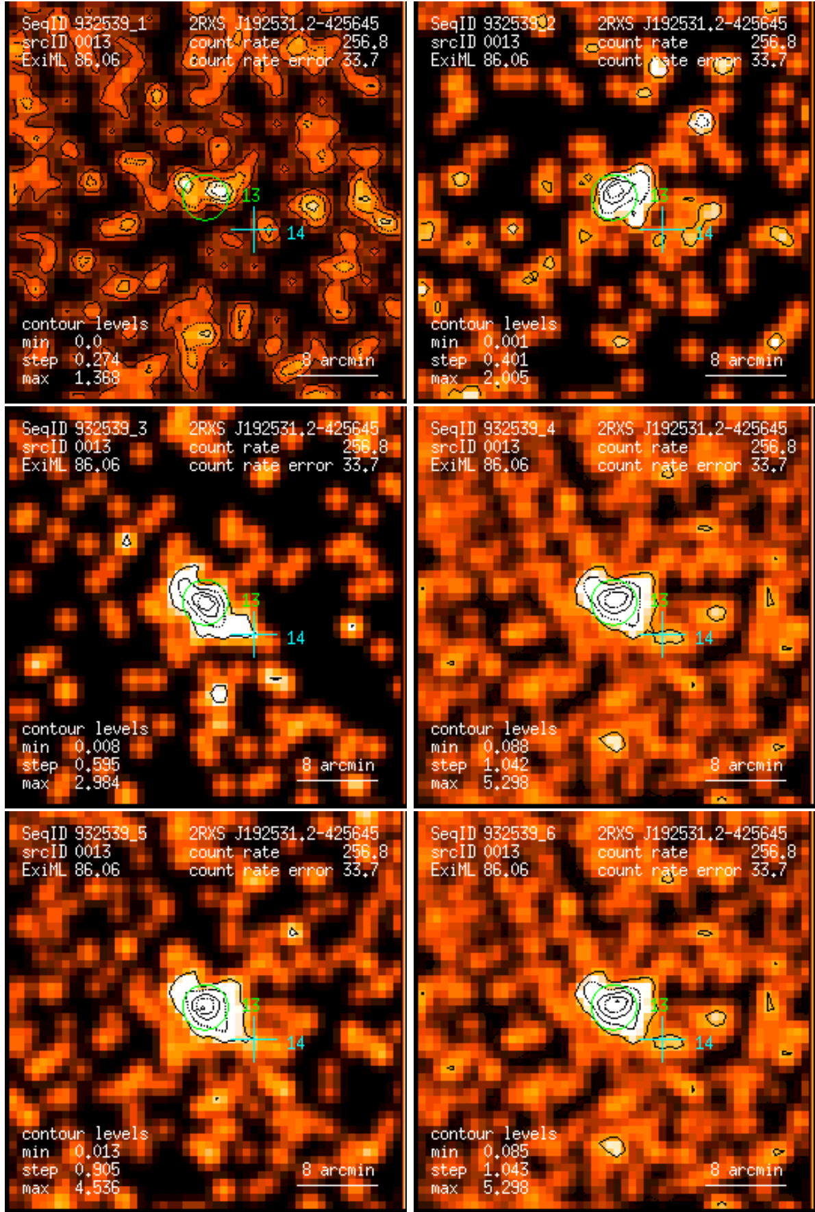
Figure 13: RASS 932539: detection 0013: band rate images, Gaussian filter: (1) PSPC channels 11 – 41, (2) 52 – 90, (3) 91 – 201, (4) 11 – 235, (5) 52 – 201, (6) 11 – 201. Broad band rates in counts/ks. Band rate contour levels in counts/ks/arcmin 2 .
