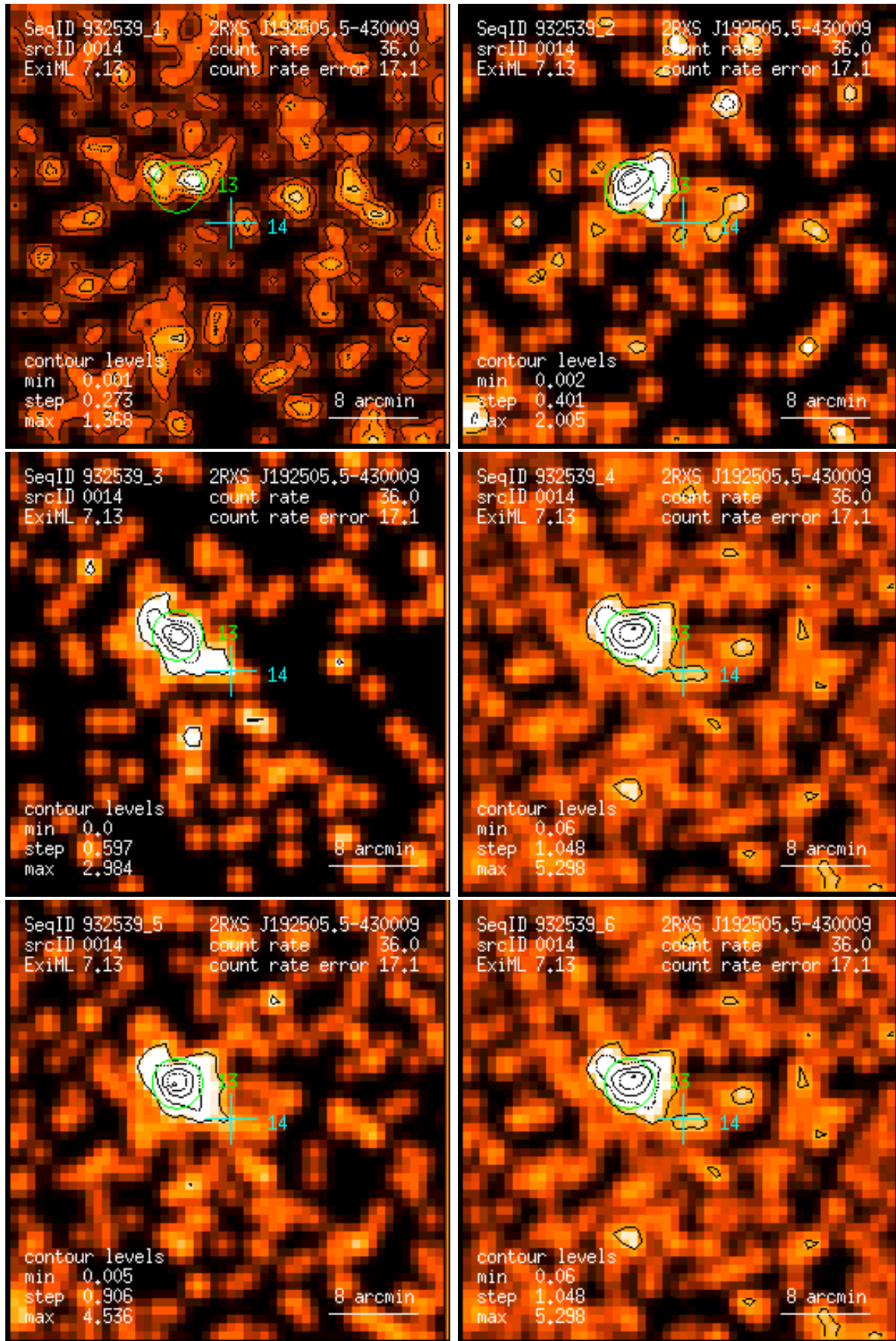
Figure 14: RASS 932539: detection 0014: band rate images, Gaussian filter: (1) PSPC channels 11 – 41, (2) 52 – 90, (3) 91 – 201, (4) 11 – 235, (5) 52 – 201, (6) 11 – 201. Broad band rates in counts/ks. Band rate contour levels in counts/ks/arcmin 2 .
