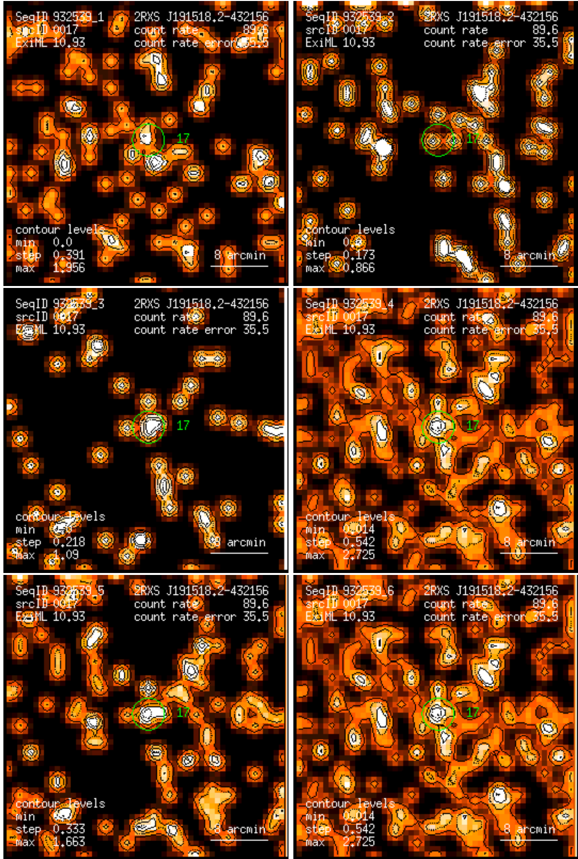
Figure 17: RASS 932539: detection 0017: band rate images, Gaussian filter: (1) PSPC channels 11 – 41, (2) 52 – 90, (3) 91 – 201, (4) 11 – 235, (5) 52 – 201, (6) 11 – 201. Broad band rates in counts/ks. Band rate contour levels in counts/ks/arcmin 2 .
