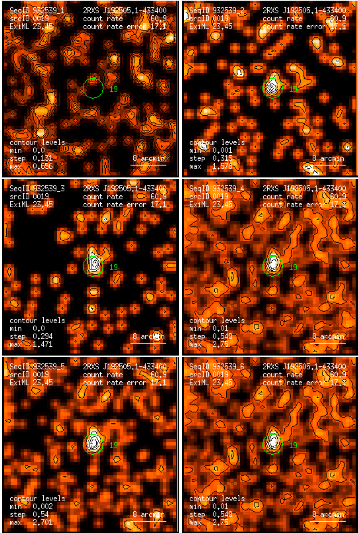
Figure 19: RASS 932539: detection 0019: band rate images, Gaussian filter: (1) PSPC channels 11 – 41, (2) 52 – 90, (3) 91 – 201, (4) 11 – 235, (5) 52 – 201, (6) 11 – 201. Broad band rates in counts/ks. Band rate contour levels in counts/ks/arcmin 2 .
