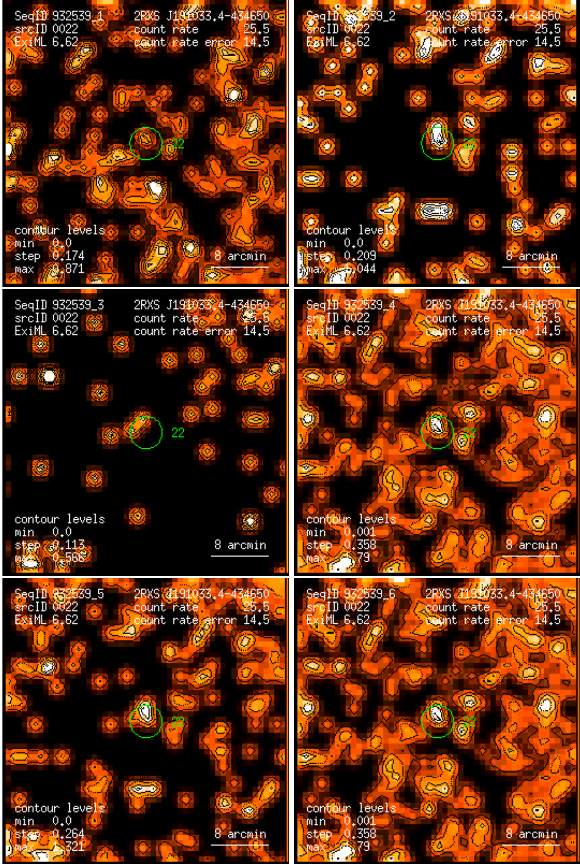
Figure 22: RASS 932539: detection 0022: band rate images, Gaussian filter: (1) PSPC channels 11 – 41, (2) 52 – 90, (3) 91 – 201, (4) 11 – 235, (5) 52 – 201, (6) 11 – 201. Broad band rates in counts/ks. Band rate contour levels in counts/ks/arcmin 2 .
