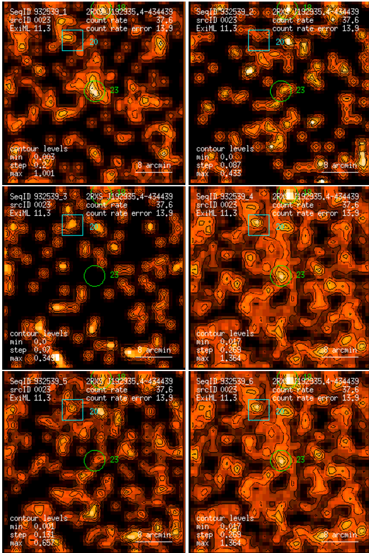
Figure 23: RASS 932539: detection 0023: band rate images, Gaussian filter: (1) PSPC channels 11 – 41, (2) 52 – 90, (3) 91 – 201, (4) 11 – 235, (5) 52 – 201, (6) 11 – 201. Broad band rates in counts/ks. Band rate contour levels in counts/ks/arcmin 2 .
