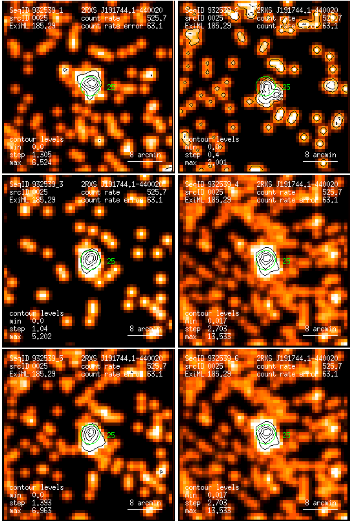
Figure 25: RASS 932539: detection 0025: band rate images, Gaussian filter: (1) PSPC channels 11 – 41, (2) 52 – 90, (3) 91 – 201, (4) 11 – 235, (5) 52 – 201, (6) 11 – 201. Broad band rates in counts/ks. Band rate contour levels in counts/ks/arcmin 2 .
