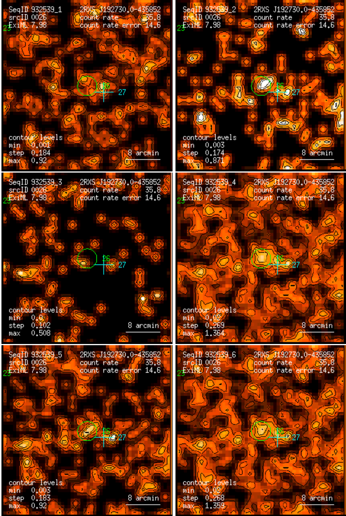
Figure 26: RASS 932539: detection 0026: band rate images, Gaussian filter: (1) PSPC channels 11 – 41, (2) 52 – 90, (3) 91 – 201, (4) 11 – 235, (5) 52 – 201, (6) 11 – 201. Broad band rates in counts/ks. Band rate contour levels in counts/ks/arcmin 2 .
