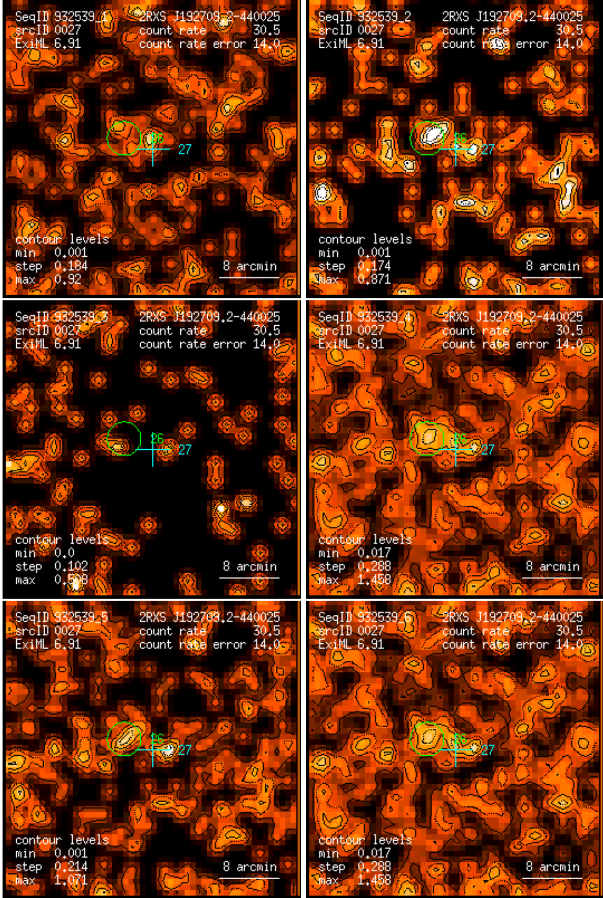
Figure 27: RASS 932539: detection 0027: band rate images, Gaussian filter: (1) PSPC channels 11 – 41, (2) 52 – 90, (3) 91 – 201, (4) 11 – 235, (5) 52 – 201, (6) 11 – 201. Broad band rates in counts/ks. Band rate contour levels in counts/ks/arcmin 2 .
