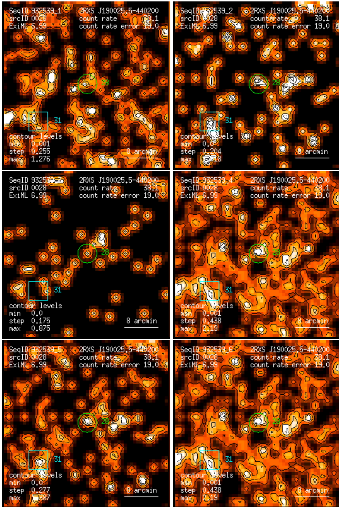
Figure 28: RASS 932539: detection 0028: band rate images, Gaussian filter: (1) PSPC channels 11 – 41, (2) 52 – 90, (3) 91 – 201, (4) 11 – 235, (5) 52 – 201, (6) 11 – 201. Broad band rates in counts/ks. Band rate contour levels in counts/ks/arcmin 2 .
