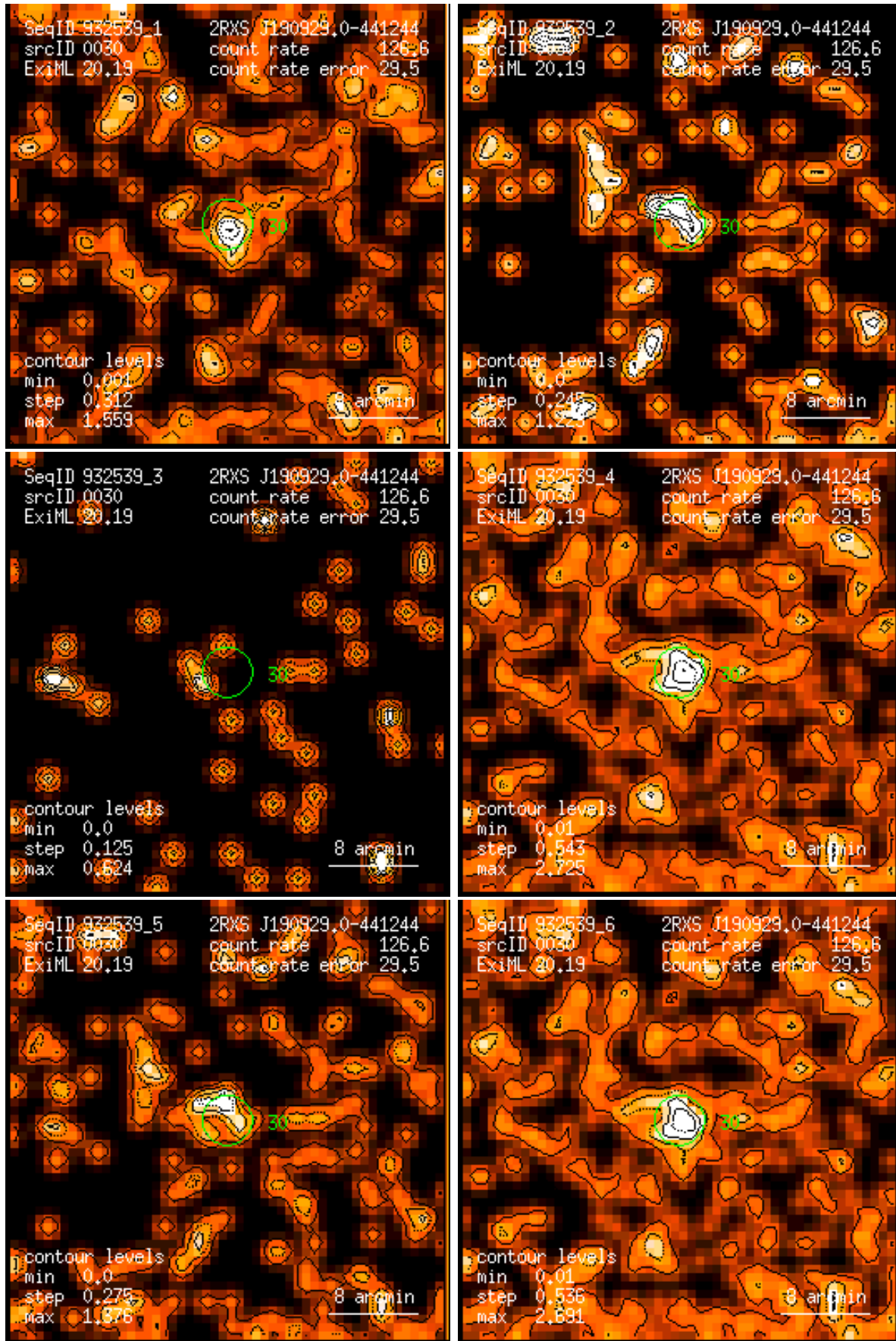
Figure 30: RASS 932539: detection 0030: band rate images, Gaussian filter: (1) PSPC channels 11 – 41, (2) 52 – 90, (3) 91 – 201, (4) 11 – 235, (5) 52 – 201, (6) 11 – 201. Broad band rates in counts/ks. Band rate contour levels in counts/ks/arcmin 2 .
