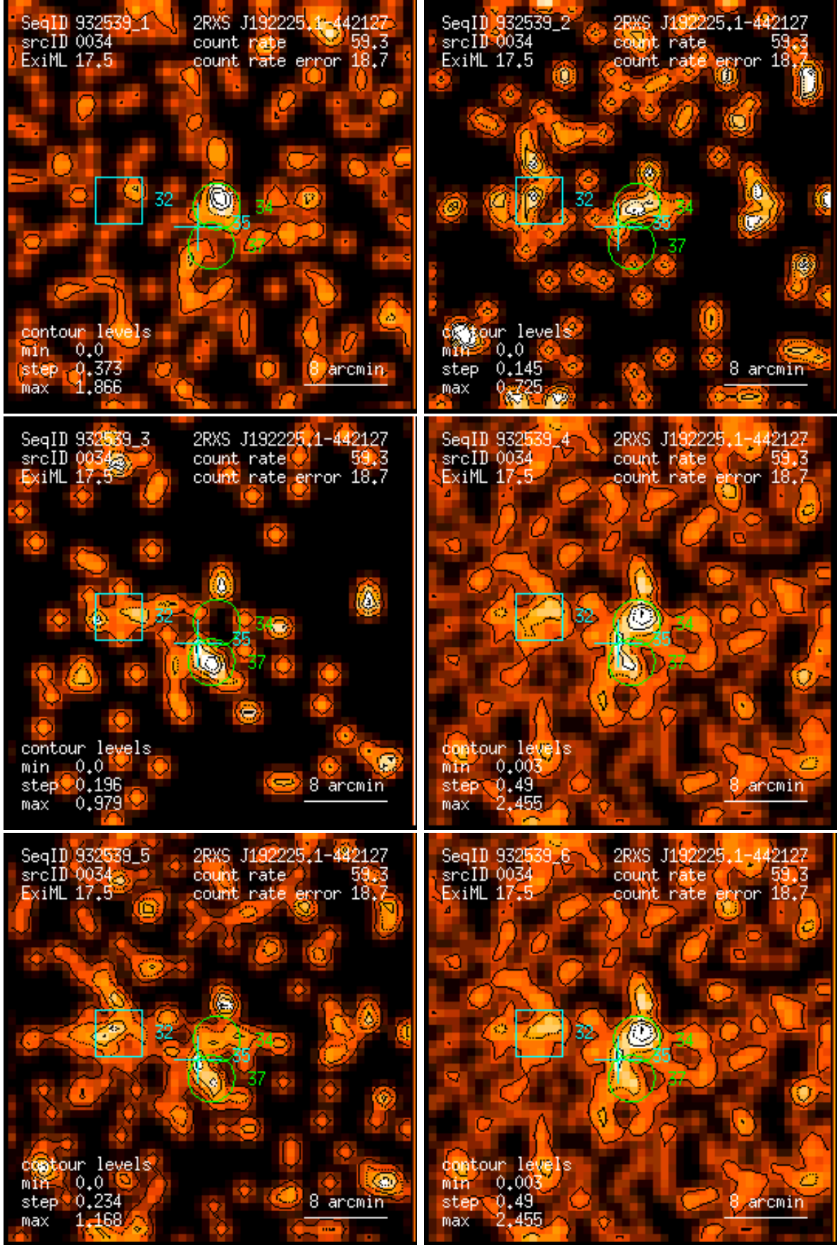
Figure 34: RASS 932539: detection 0034: band rate images, Gaussian filter: (1) PSPC channels 11 – 41, (2) 52 – 90, (3) 91 – 201, (4) 11 – 235, (5) 52 – 201, (6) 11 – 201. Broad band rates in counts/ks. Band rate contour levels in counts/ks/arcmin 2 .
