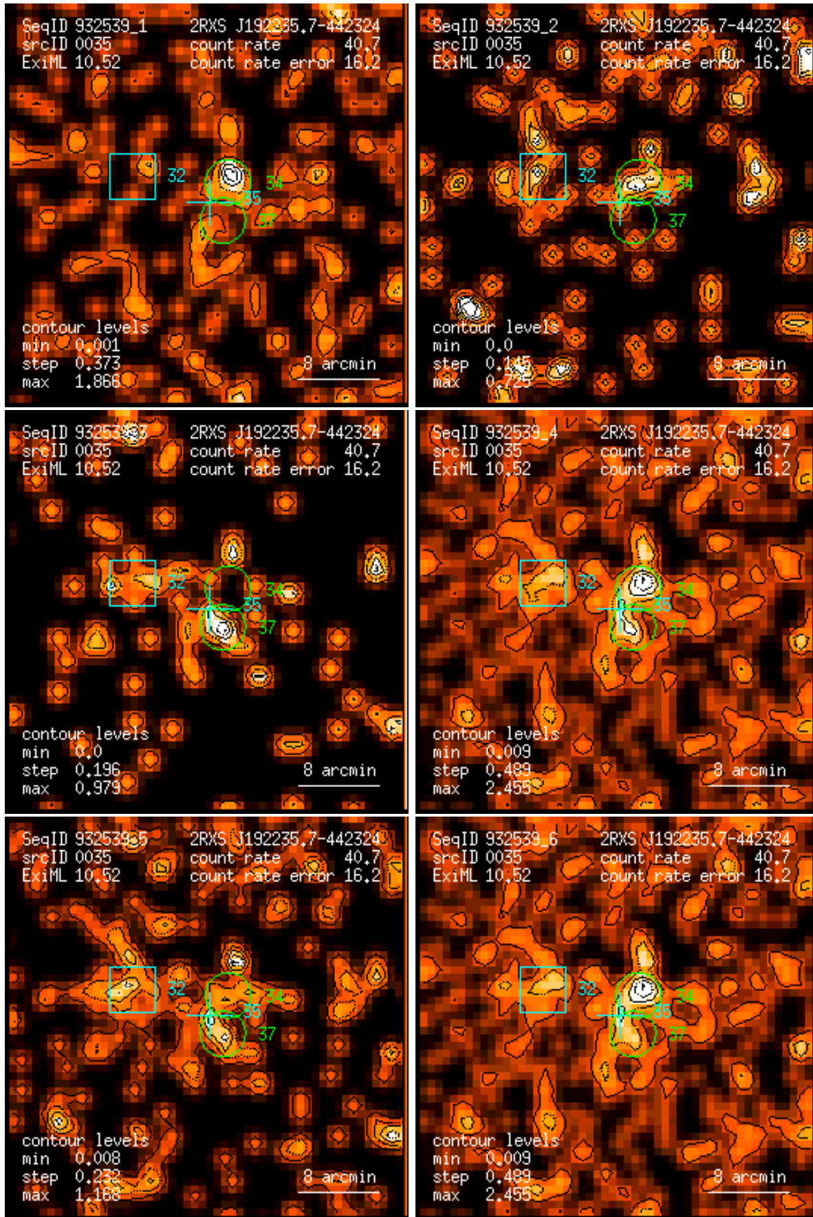
Figure 35: RASS 932539: detection 0035: band rate images, Gaussian filter: (1) PSPC channels 11 – 41, (2) 52 – 90, (3) 91 – 201, (4) 11 – 235, (5) 52 – 201, (6) 11 – 201. Broad band rates in counts/ks. Band rate contour levels in counts/ks/arcmin 2 .
