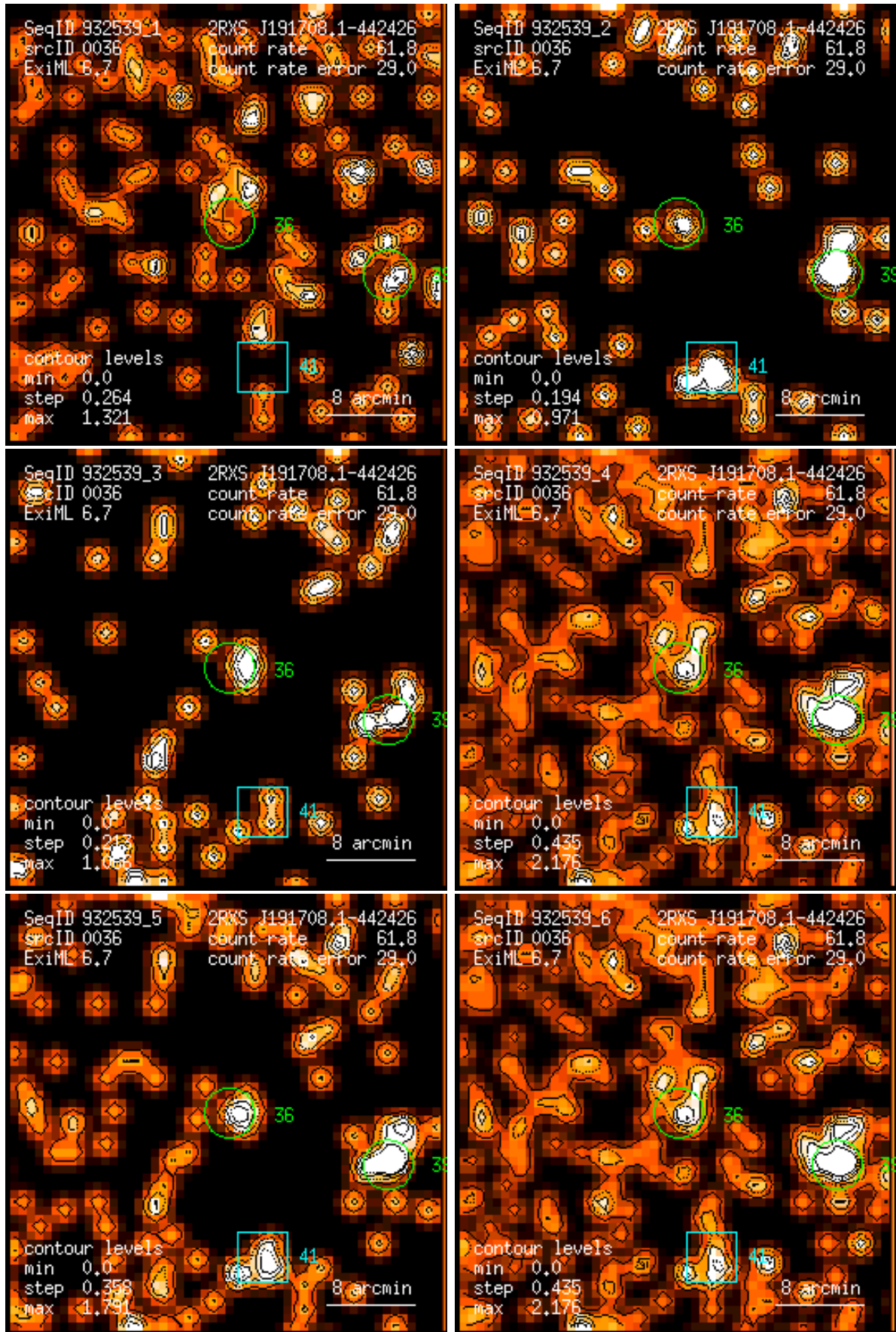
Figure 36: RASS 932539: detection 0036: band rate images, Gaussian filter: (1) PSPC channels 11 – 41, (2) 52 – 90, (3) 91 – 201, (4) 11 – 235, (5) 52 – 201, (6) 11 – 201. Broad band rates in counts/ks. Band rate contour levels in counts/ks/arcmin 2 .
