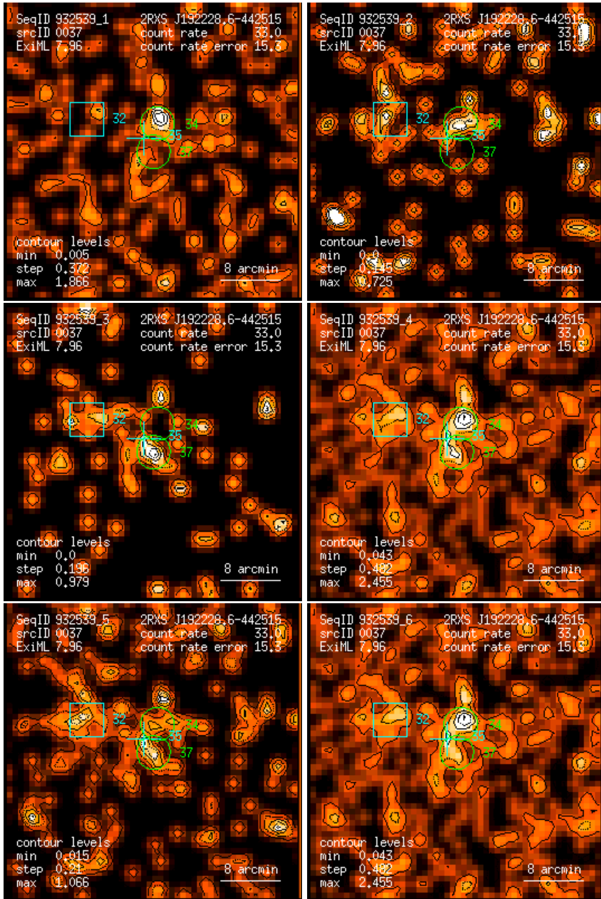
Figure 37: RASS 932539: detection 0037: band rate images, Gaussian filter: (1) PSPC channels 11 – 41, (2) 52 – 90, (3) 91 – 201, (4) 11 – 235, (5) 52 – 201, (6) 11 – 201. Broad band rates in counts/ks. Band rate contour levels in counts/ks/arcmin 2 .
