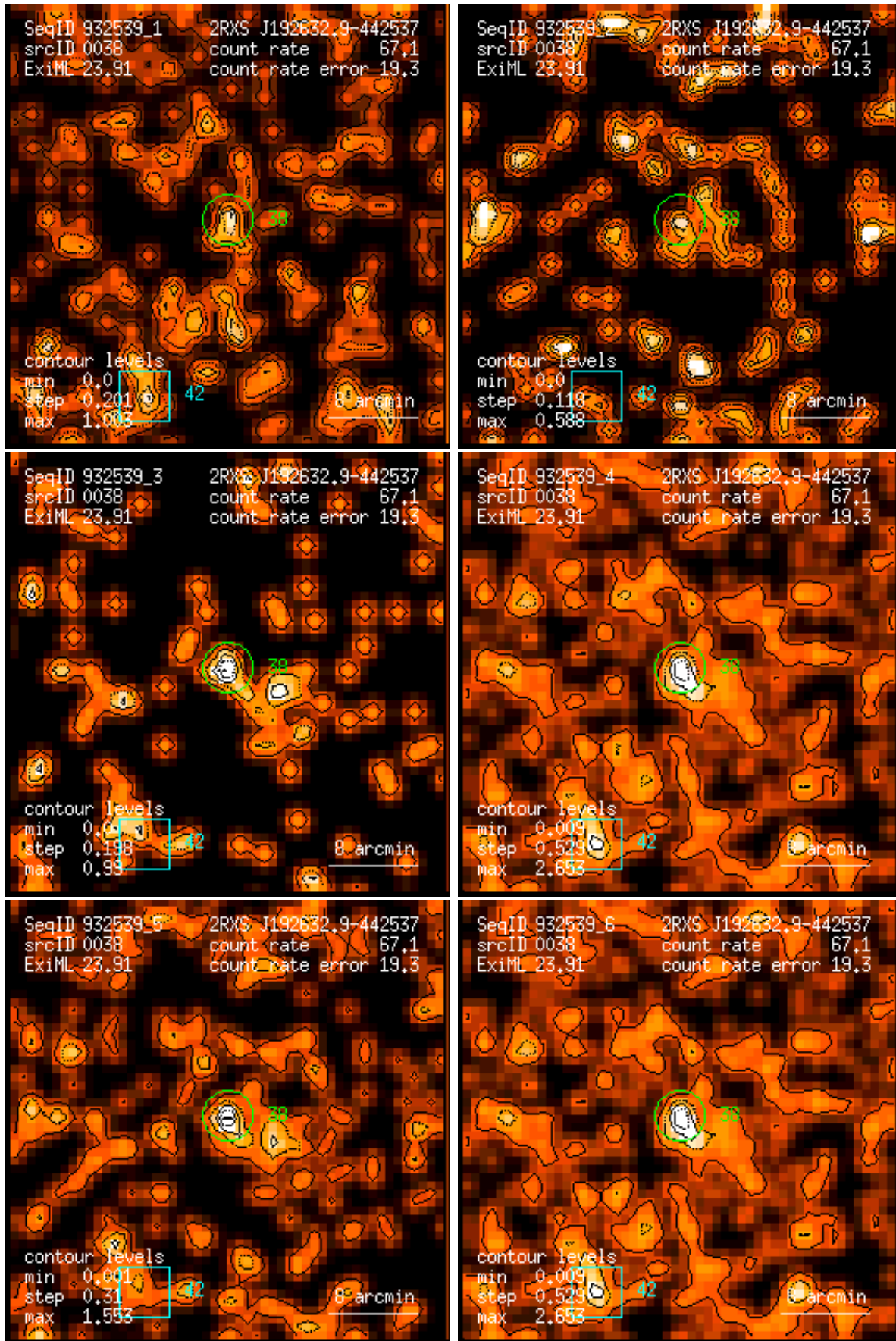
Figure 38: RASS 932539: detection 0038: band rate images, Gaussian filter: (1) PSPC channels 11 – 41, (2) 52 – 90, (3) 91 – 201, (4) 11 – 235, (5) 52 – 201, (6) 11 – 201. Broad band rates in counts/ks. Band rate contour levels in counts/ks/arcmin 2 .
