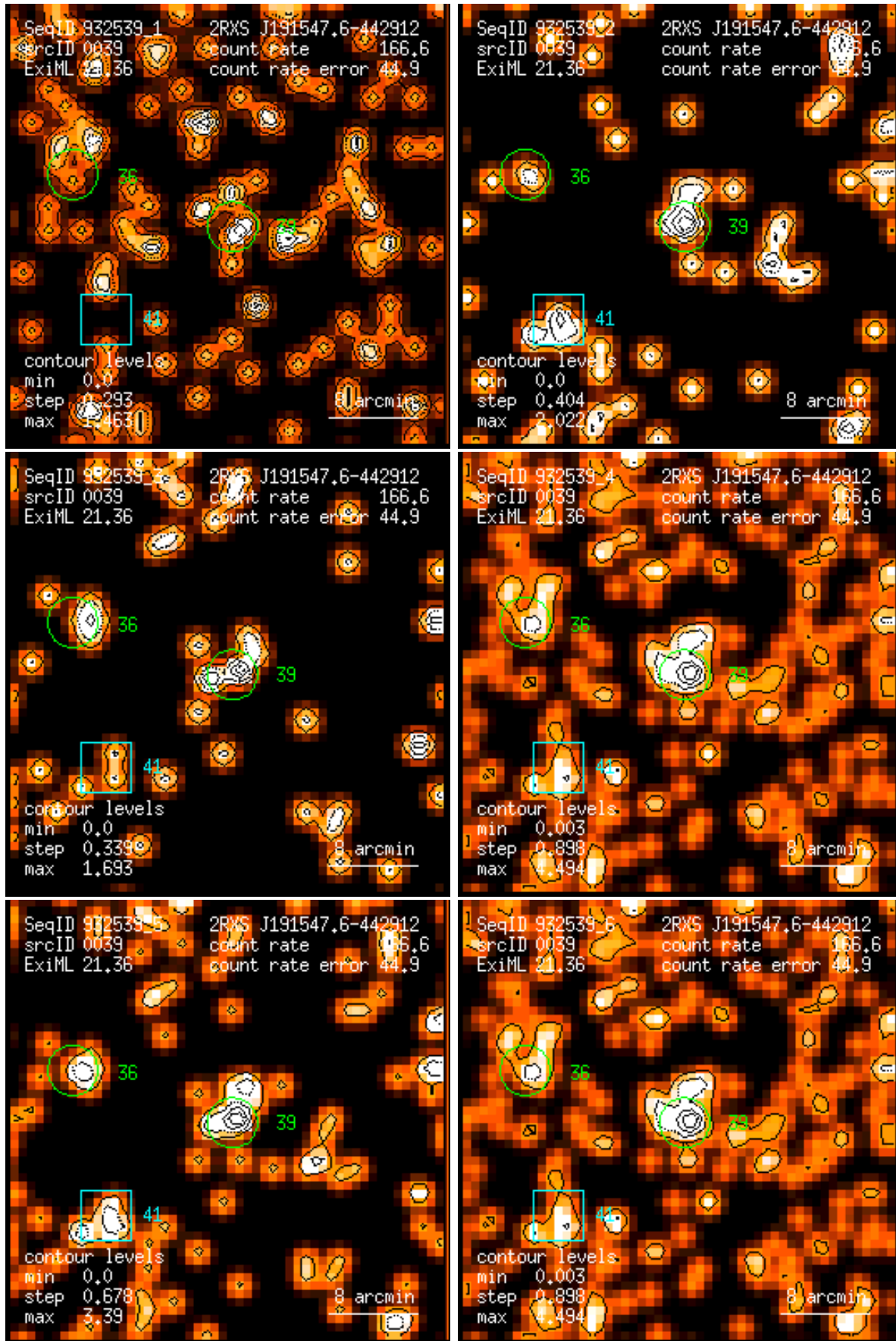
Figure 39: RASS 932539: detection 0039: band rate images, Gaussian filter: (1) PSPC channels 11 – 41, (2) 52 – 90, (3) 91 – 201, (4) 11 – 235, (5) 52 – 201, (6) 11 – 201. Broad band rates in counts/ks. Band rate contour levels in counts/ks/arcmin 2 .
