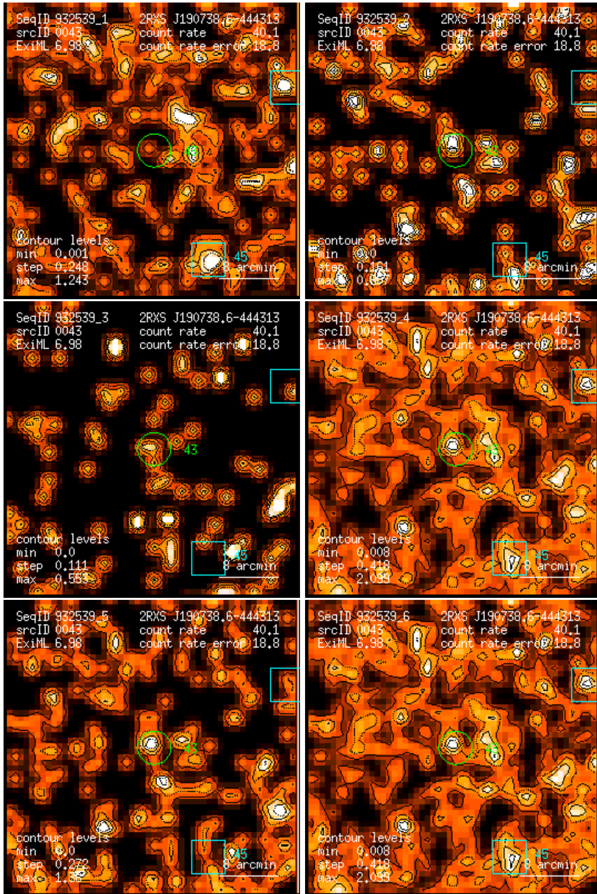
Figure 43: RASS 932539: detection 0043: band rate images, Gaussian filter: (1) PSPC channels 11 – 41, (2) 52 – 90, (3) 91 – 201, (4) 11 – 235, (5) 52 – 201, (6) 11 – 201. Broad band rates in counts/ks. Band rate contour levels in counts/ks/arcmin 2 .
