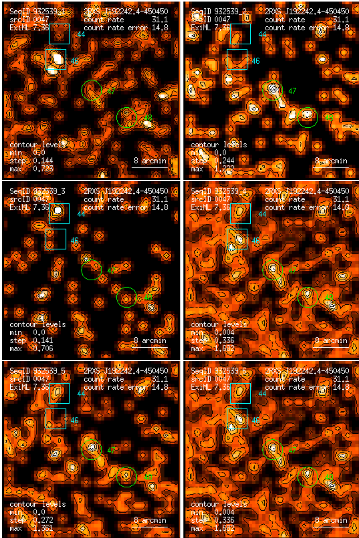
Figure 47: RASS 932539: detection 0047: band rate images, Gaussian filter: (1) PSPC channels 11 – 41, (2) 52 – 90, (3) 91 – 201, (4) 11 – 235, (5) 52 – 201, (6) 11 – 201. Broad band rates in counts/ks. Band rate contour levels in counts/ks/arcmin 2 .
