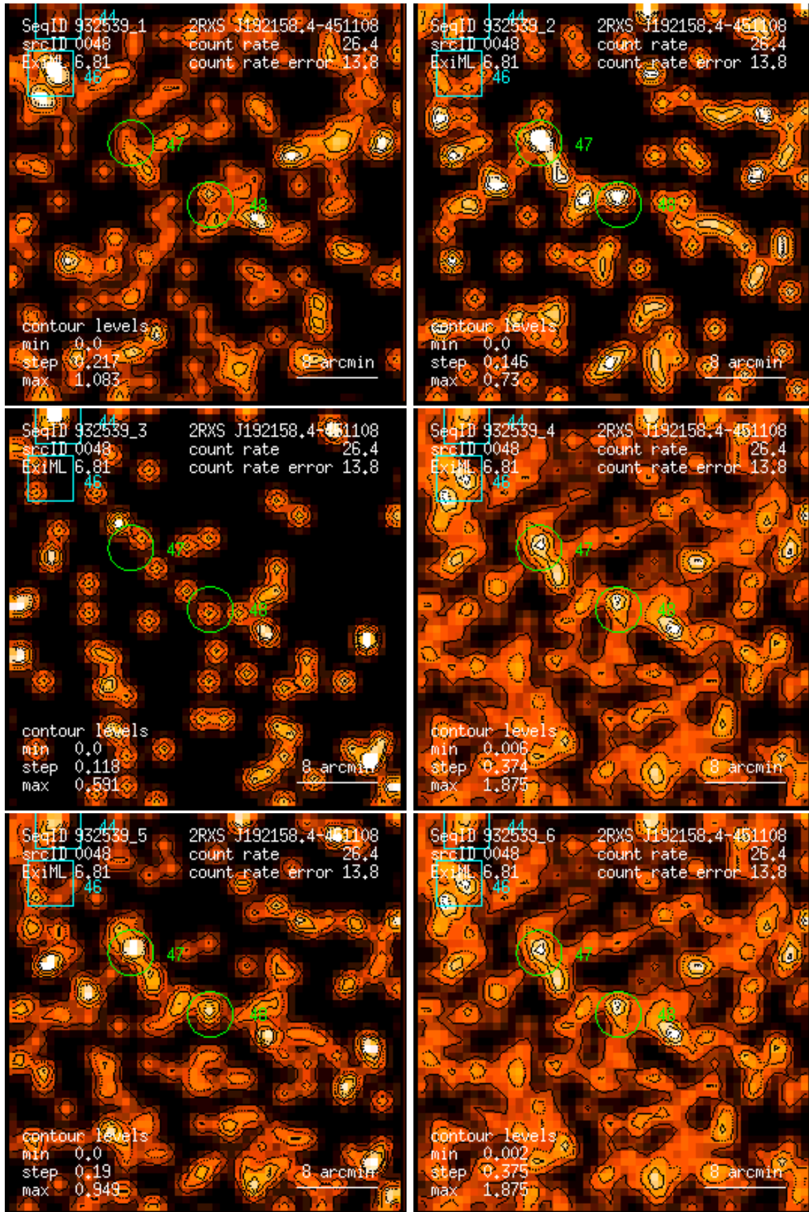
Figure 48: RASS 932539: detection 0048: band rate images, Gaussian filter: (1) PSPC channels 11 – 41, (2) 52 – 90, (3) 91 – 201, (4) 11 – 235, (5) 52 – 201, (6) 11 – 201. Broad band rates in counts/ks. Band rate contour levels in counts/ks/arcmin 2 .
