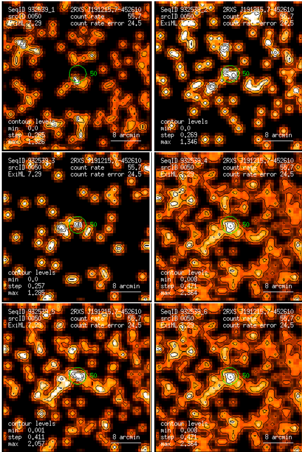
Figure 50: RASS 932539: detection 0050: band rate images, Gaussian filter: (1) PSPC channels 11 – 41, (2) 52 – 90, (3) 91 – 201, (4) 11 – 235, (5) 52 – 201, (6) 11 – 201. Broad band rates in counts/ks. Band rate contour levels in counts/ks/arcmin 2 .
