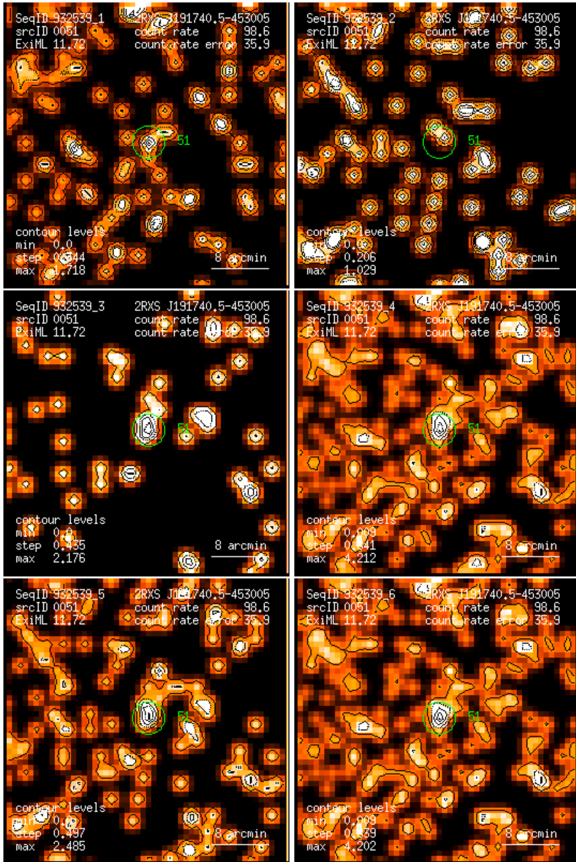
Figure 51: RASS 932539: detection 0051: band rate images, Gaussian filter: (1) PSPC channels 11 – 41, (2) 52 – 90, (3) 91 – 201, (4) 11 – 235, (5) 52 – 201, (6) 11 – 201. Broad band rates in counts/ks. Band rate contour levels in counts/ks/arcmin 2 .
