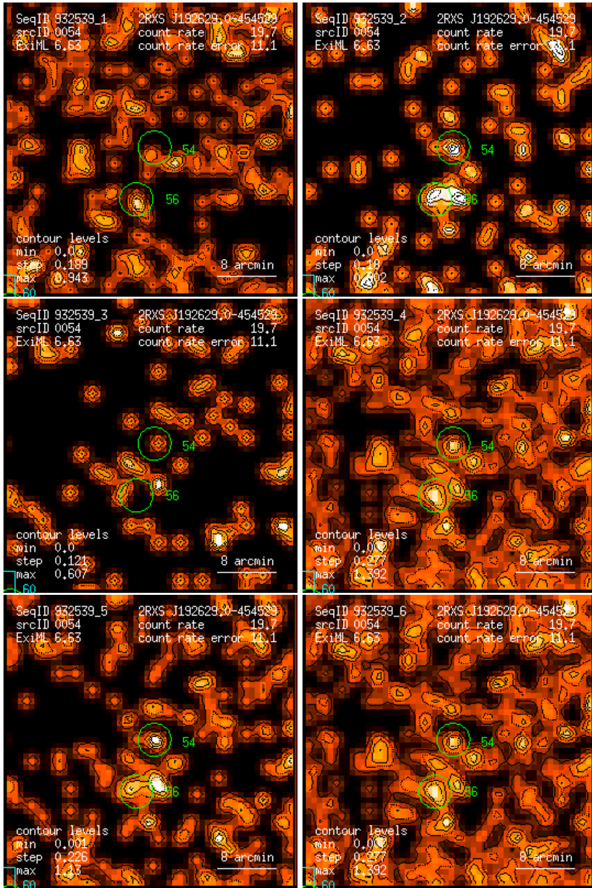
Figure 54: RASS 932539: detection 0054: band rate images, Gaussian filter: (1) PSPC channels 11 – 41, (2) 52 – 90, (3) 91 – 201, (4) 11 – 235, (5) 52 – 201, (6) 11 – 201. Broad band rates in counts/ks. Band rate contour levels in counts/ks/arcmin 2 .
