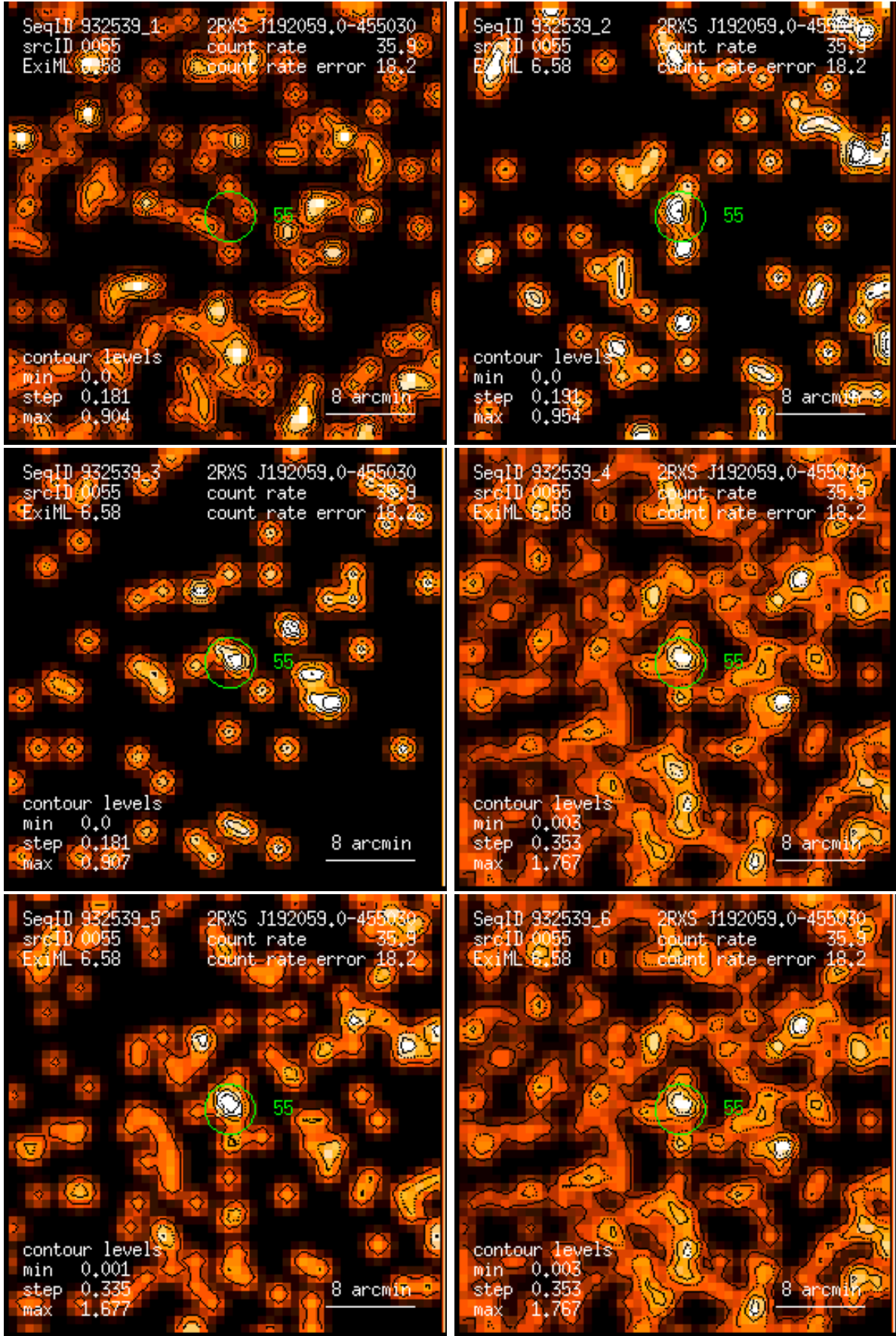
Figure 55: RASS 932539: detection 0055: band rate images, Gaussian filter: (1) PSPC channels 11 – 41, (2) 52 – 90, (3) 91 – 201, (4) 11 – 235, (5) 52 – 201, (6) 11 – 201. Broad band rates in counts/ks. Band rate contour levels in counts/ks/arcmin 2 .
