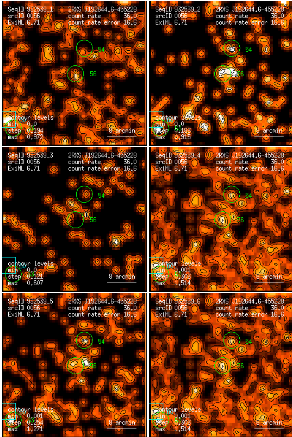
Figure 56: RASS 932539: detection 0056: band rate images, Gaussian filter: (1) PSPC channels 11 – 41, (2) 52 – 90, (3) 91 – 201, (4) 11 – 235, (5) 52 – 201, (6) 11 – 201. Broad band rates in counts/ks. Band rate contour levels in counts/ks/arcmin 2 .
