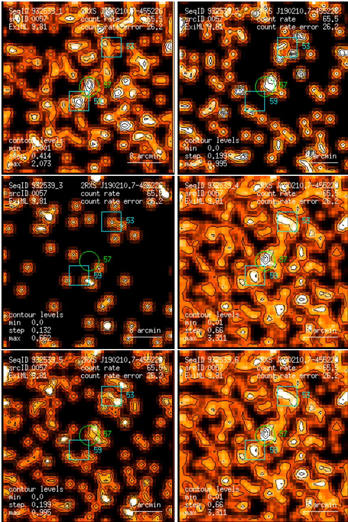
Figure 57: RASS 932539: detection 0057: band rate images, Gaussian filter: (1) PSPC channels 11 – 41, (2) 52 – 90, (3) 91 – 201, (4) 11 – 235, (5) 52 – 201, (6) 11 – 201. Broad band rates in counts/ks. Band rate contour levels in counts/ks/arcmin 2 .
