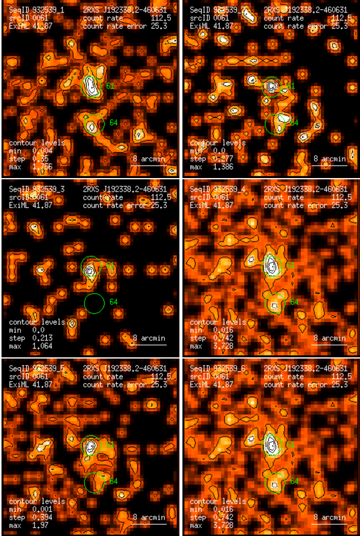
Figure 61: RASS 932539: detection 0061: band rate images, Gaussian filter: (1) PSPC channels 11 – 41, (2) 52 – 90, (3) 91 – 201, (4) 11 – 235, (5) 52 – 201, (6) 11 – 201. Broad band rates in counts/ks. Band rate contour levels in counts/ks/arcmin 2 .
