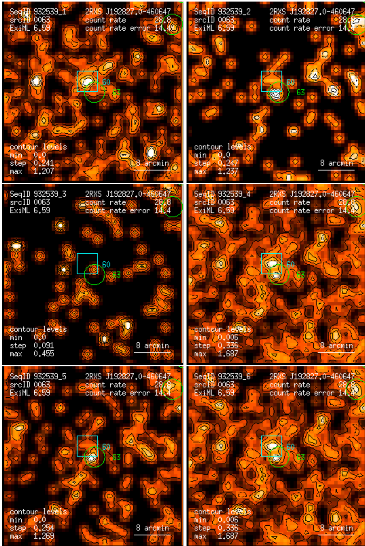
Figure 63: RASS 932539: detection 0063: band rate images, Gaussian filter: (1) PSPC channels 11 – 41, (2) 52 – 90, (3) 91 – 201, (4) 11 – 235, (5) 52 – 201, (6) 11 – 201. Broad band rates in counts/ks. Band rate contour levels in counts/ks/arcmin 2 .
