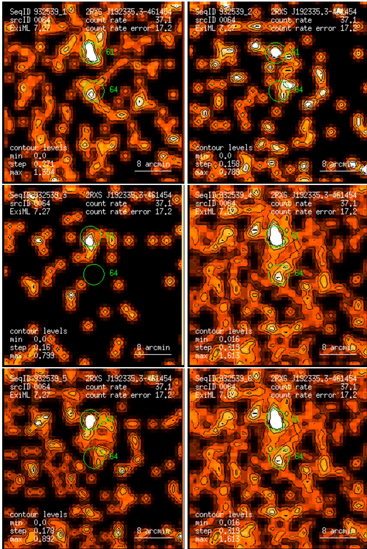
Figure 64: RASS 932539: detection 0064: band rate images, Gaussian filter: (1) PSPC channels 11 – 41, (2) 52 – 90, (3) 91 – 201, (4) 11 – 235, (5) 52 – 201, (6) 11 – 201. Broad band rates in counts/ks. Band rate contour levels in counts/ks/arcmin 2 .
